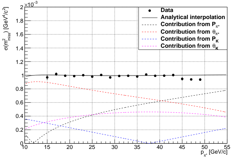
Figure 9: Gaussian resolution of the m_{miss}^2 measured on a K^+ \rightarrow \pi^+\pi^0 sample, as a function of pion momentum. The black solid line is an analytical interpolation using the expected resolutions for GTK and STRAW. The dashed lines correspond to the contributions of the individual quantities entering in the computation of m_{miss}^2 .
