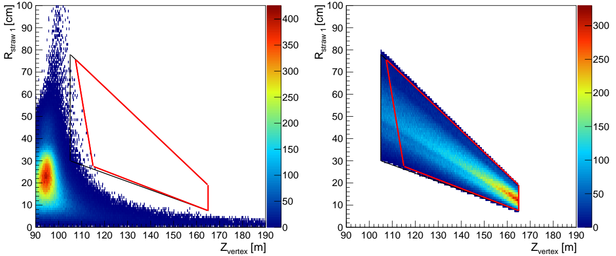
Figure 6: MC distribution of the distance of the \pi^+ track from the beam at first STRAW chamber as a function of the z coordinate of the vertex formed by the \pi^+ with a matched track in GTK, for K^+ early decays (left) and signal event (right) both with 15 < p_{\pi^+} < 35 GeV/c. Events outside the red lines are rejected by the cuts on R_{Straw1} versus Z_{vertex} applied in the \pi\nu\nu selection and described in the text. The black line following the expected profile of \pi\nu\nu events is also drawn.
