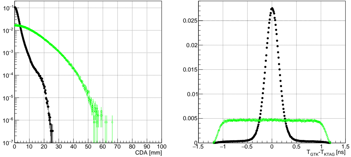
Figure 4: Left: CDA distribution of the vertex formed by a good K^+ and a \pi^+ track selected from K^+ \rightarrow \pi^+ \pi^+ \pi^- events (black dots); Right: distribution of the time difference between GTK and KTAG time candidates for K^+ and \pi^+ selected from K^+ \rightarrow \pi^+ \pi^+ \pi^- events (black dots); green dots are the same quantities computed with a random beam track instead of K^+ track.
