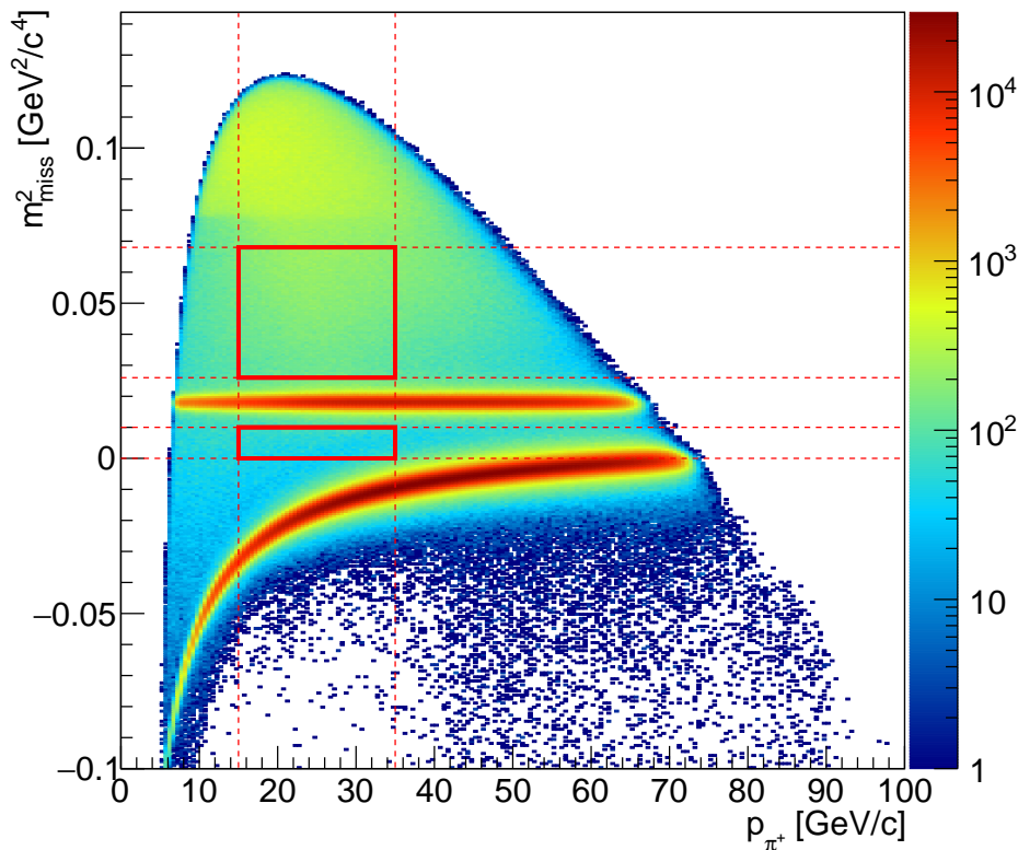
Figure 7: Distribution of m_{miss}^2 as a function of pion momentum for kaon events selected on control data. The signal regions (red box) in the (m_{miss}^2, p_{\pi^+}) plane are drawn for reference.
