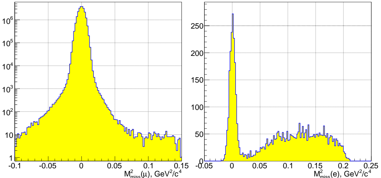
Figure 19: Squared missing mass spectra of the K^+ \rightarrow \mu^+\nu (left) and K^+ \rightarrow e^+\nu (right) decays reconstructed from 2015 minimum bias data. The backgrounds in the regions of large missing mass are low, leading to record sensitivities to HNL production.
