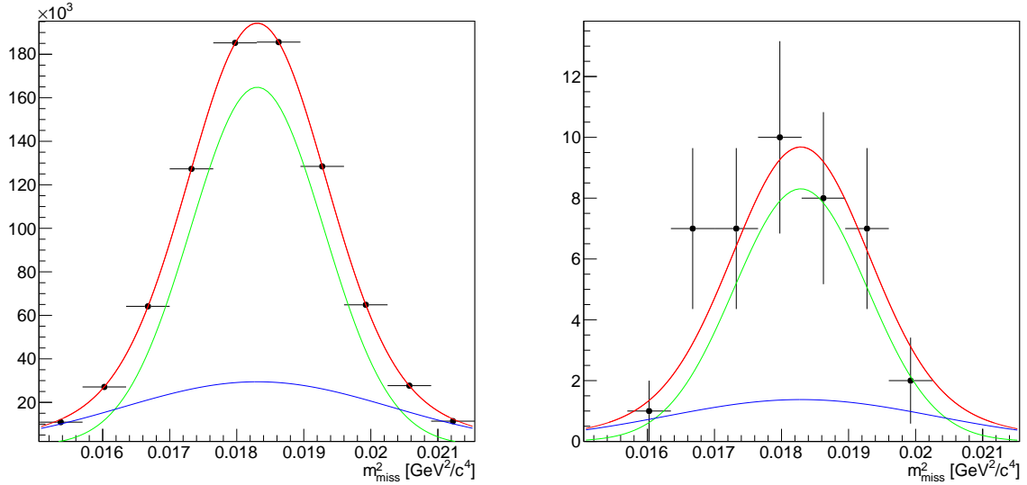
Figure 13: Distribution of events in the \pi\pi region before (left) and after (right) photon rejection. Events before photon rejection are from control trigger and must be multiplied by the downscaling factor (400) to get the total number of K^+ \rightarrow \pi^+\pi^0 before photon rejection. The 2-gaussian fit is superimposed. The overall scale is the only free parameter in the fit of the events after photon rejection, the other parameters are fixed to the value obtained by the fit before photon rejection.
