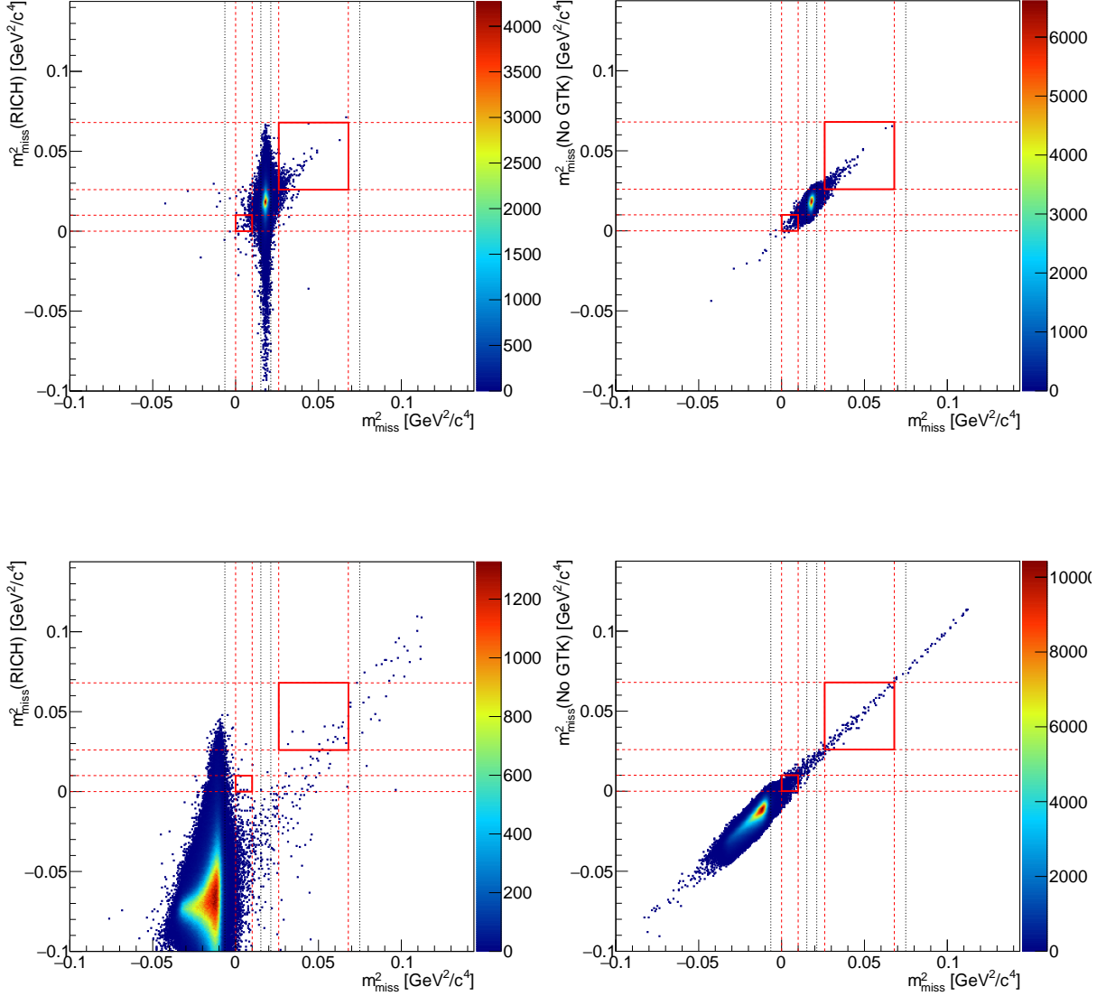
Figure 8: Top-row: distribution of m_{miss}^2(RICH) vs m_{miss}^2 (left) and m_{miss}^2(No\ GTK) vs m_{miss}^2 (right) for K^+ \rightarrow \pi^+\pi^0 events selected for kinematic studies. Bottom-row: same distribution for K^+ \rightarrow \mu^+\nu . The red tick boxes correspond to the two-dimensional projections of the signal region; the light dashed black line to the kinematical limiting line defining K^+ \rightarrow \mu^+\nu , K^+ \rightarrow \pi^+\pi^0 and K^+ \rightarrow \pi^+\pi^+\pi^- regions.
