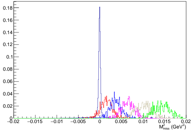
Figure 15: Distribution of the squared missing mass evaluated from one photon and one \pi^+ from K^+ decays, Eq. 14: data from \pi^0 \rightarrow \gamma\gamma events in which one photon is assumed to be undetected according to the expected inefficiency (black line) is compared with the expected spectra from \pi^0 \rightarrow A'\gamma , for A' masses from 40 to 120 MeV in 20-MeV steps (red to green lines).
