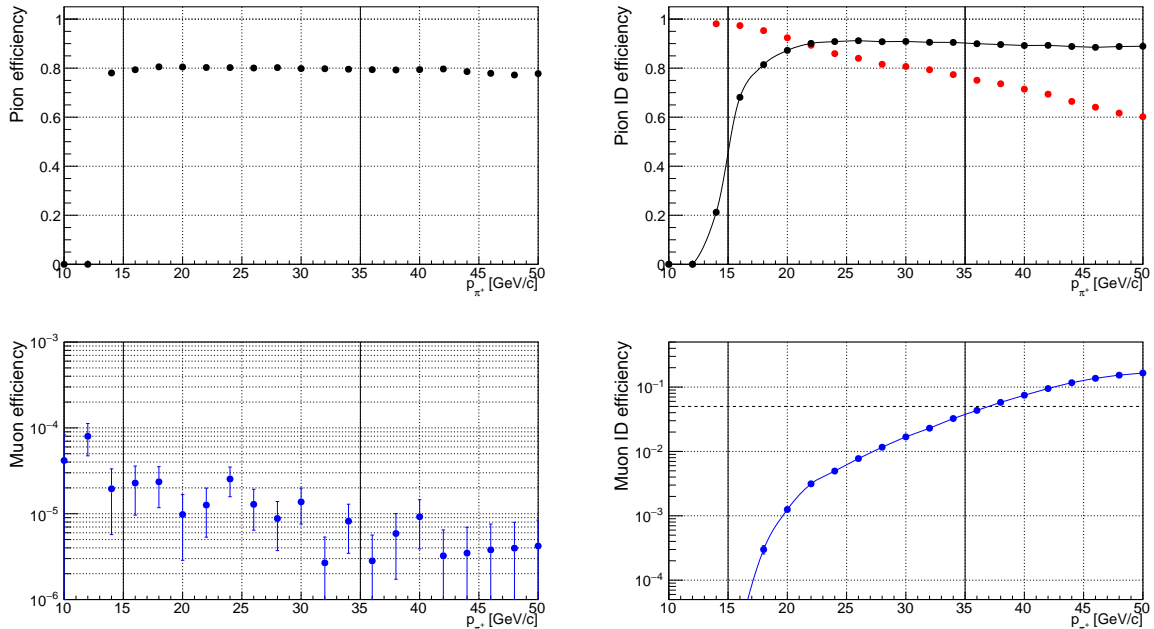
Figure 10: Left column: efficiency of pion (top) and muon (bottom) identification after requiring pion identification with calorimeters and MUV3. Right column: efficiency of standalone ring reconstruction (top black dots), pion (top red dots) and muon (bottom) identification after applying the \pi^+ ID condition described in the text on the reconstructed mass from standalone ring.
