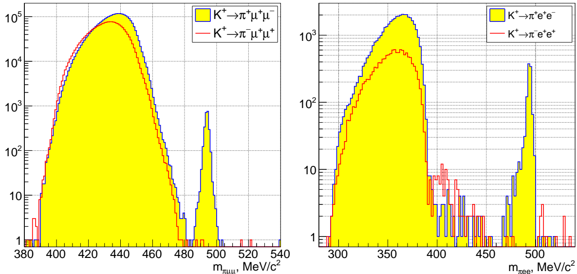
Figure 18: Reconstructed \pi\ell\ell mass spectra obtained from a partial 2016 data sample with selections for the rare decays K^+ \rightarrow \pi^+\ell^+\ell^- and forbidden LNV decays K^+ \rightarrow \pi^-\ell^+\ell^+ .
