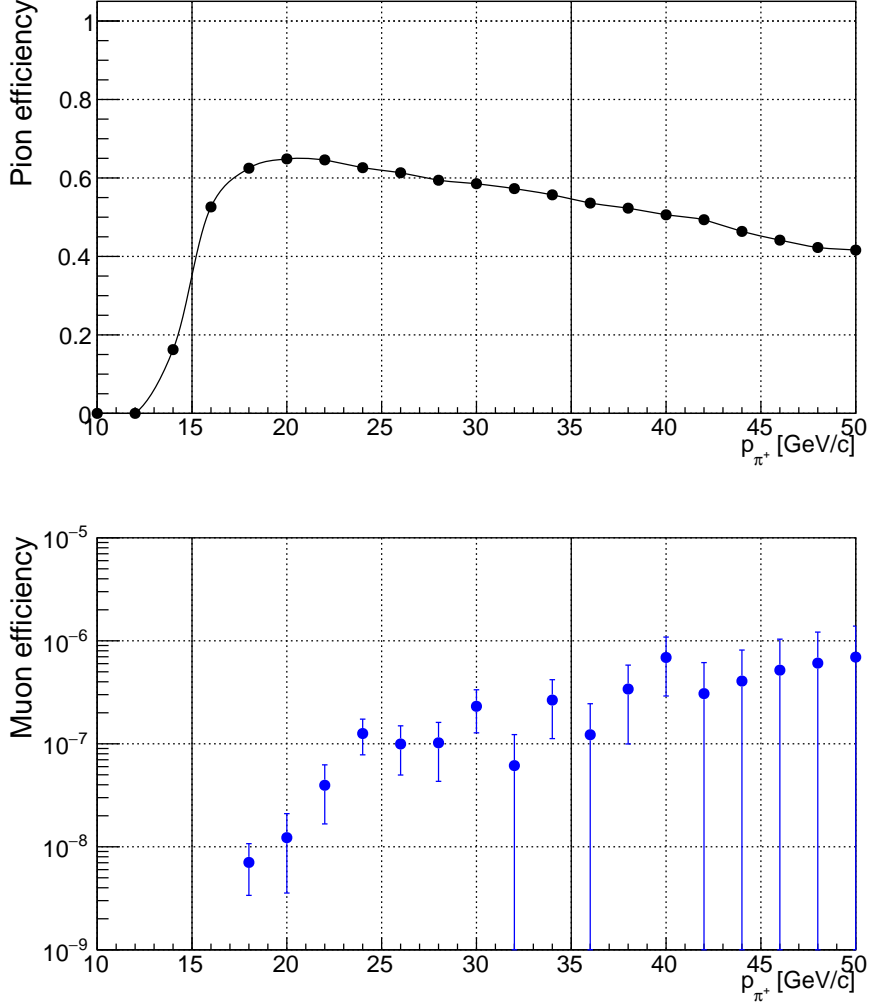
Figure 11: Combined pion (top) and muon efficiency (bottom) after pion identification in calorimeter and RICH, assuming that the two detectors are independent.
