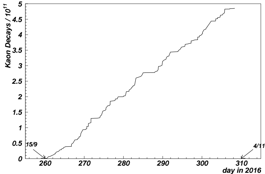
Figure 2: Integrated number of kaon decays in the 60 m long fiducial volume collected in sample A, obtained from reconstructed K^+ \rightarrow \pi^+\pi^+\pi^- decays in the control trigger stream.
