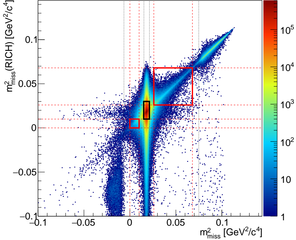
Figure 12: Distribution in the (m_{miss}^2(RICH), m_{miss}^2) plane of events triggered by the PNN trigger line and passing the \pi\nu\nu selection before the photon rejection and with 15 < p_{\pi^+} < 35 GeV/c. The signal regions (red tick box) and the \pi\pi region (black tick box) are drawn.
