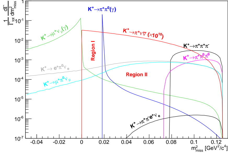
Figure 3: Theoretical m_{miss}^2 distribution for signal and backgrounds of the main K^+ decay modes: the backgrounds are normalized according to their branching ratio; the signal is multiplied by a factor 10^{10} .
