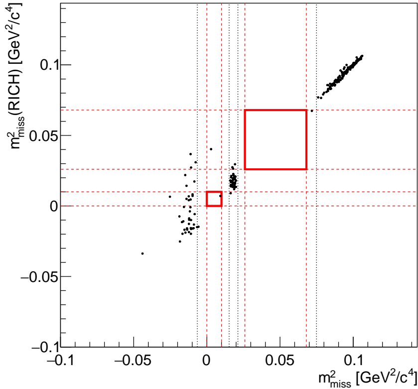
Figure 14: Distribution in the (m_{miss}^2(RICH), m_{miss}^2) plane of PNN triggered events passing the \pi\nu\nu selection, except for the cut on m_{miss}^2(No - GTK) (Section 7.5). Signal regions (red tick boxes) and lines defining the background regions (light dashed lines) are drawn. The event apparently left in region 1 has m_{miss}^2(No - GTK) outside the signal region.
