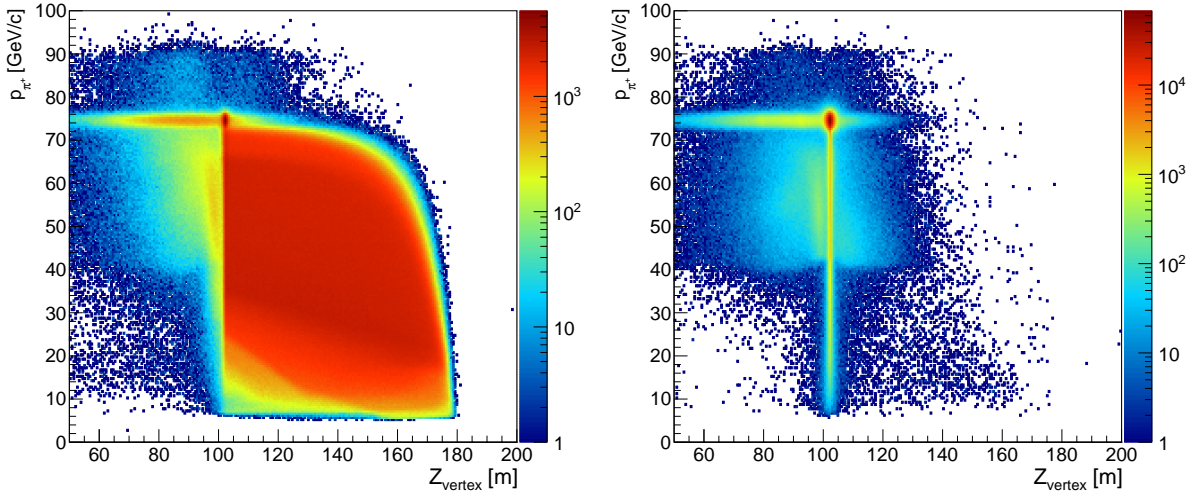
Figure 5: Distribution of \pi^+ momentum as a function of the z coordinate of the vertex for kaon events (left) and non kaon events (right); kaon and non kaon events are defined in the text.
