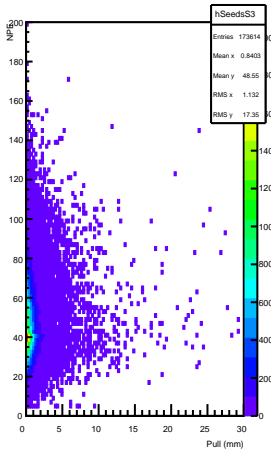
Seed Pull vs NPE Station 3
