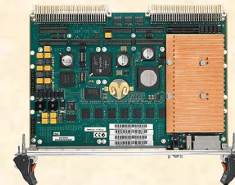
PMC card and carrier (VMEbus)
