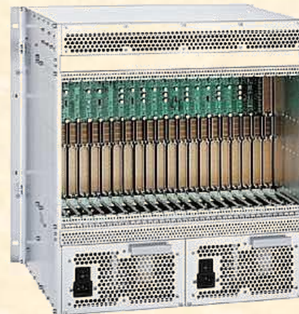
6U CompactPCI chassis and card
