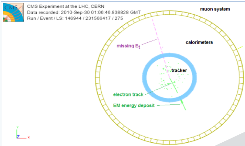
Sample W boson candidate: x-y view of detector cross-section
