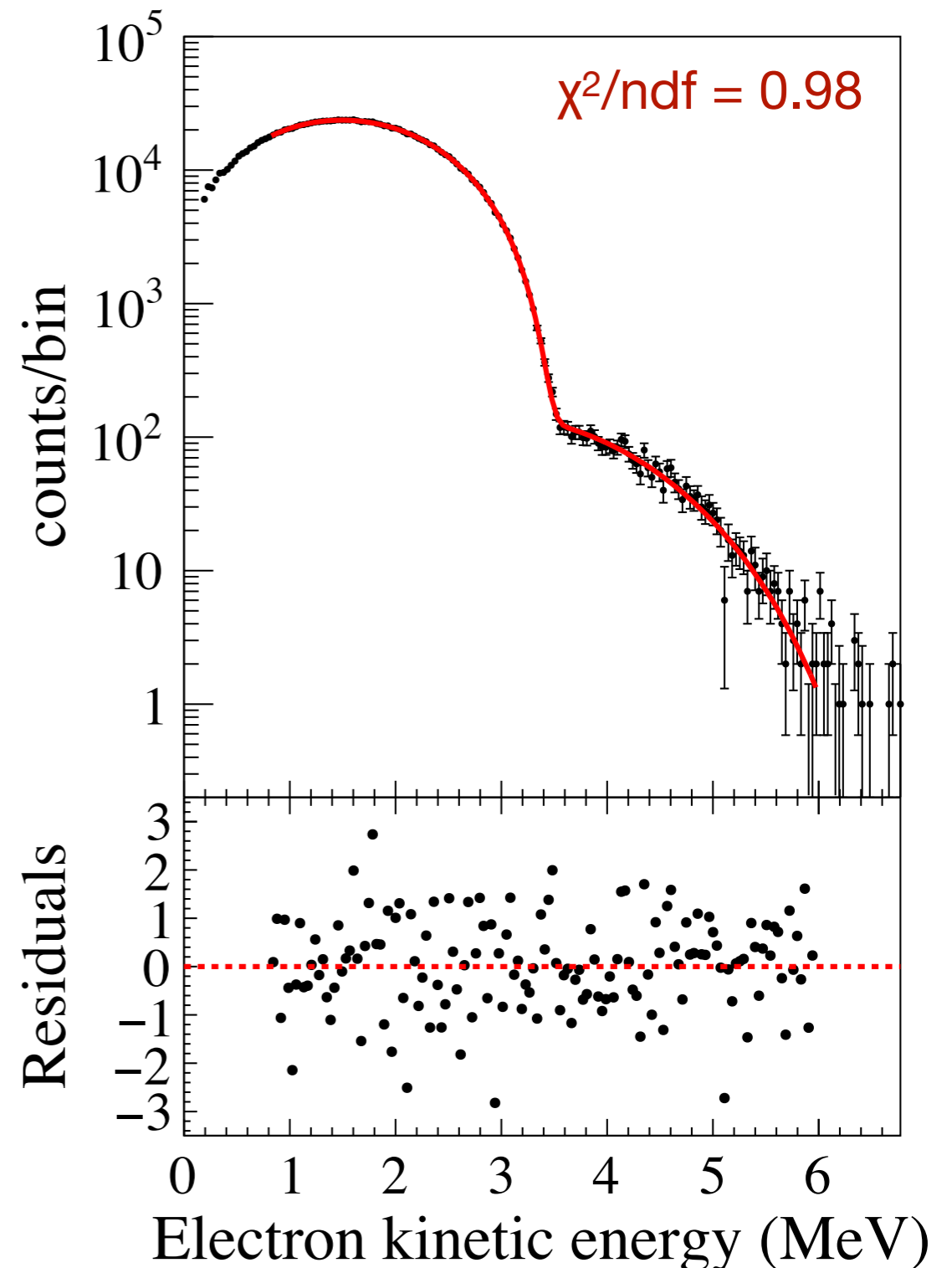
Typical Fit to the Background Subtracted \beta -energy Spectrum Measured with the CsI(Na) Detector
