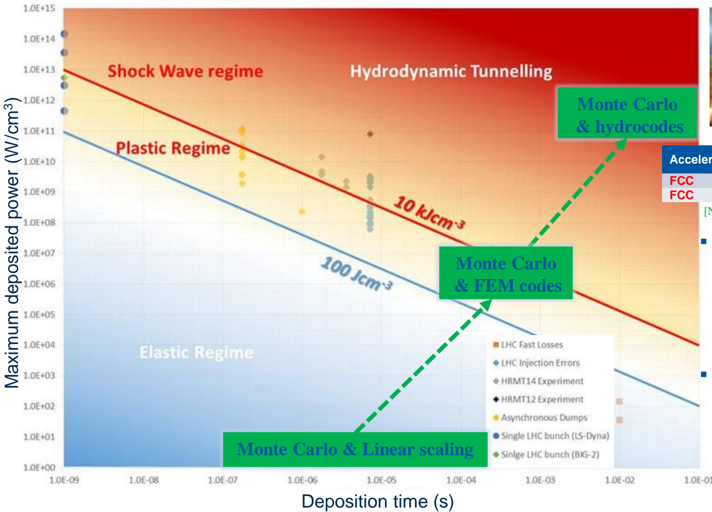
Mechanical responses in different regimes [A. Bertarelli, Joint Accelerator School 2014]
