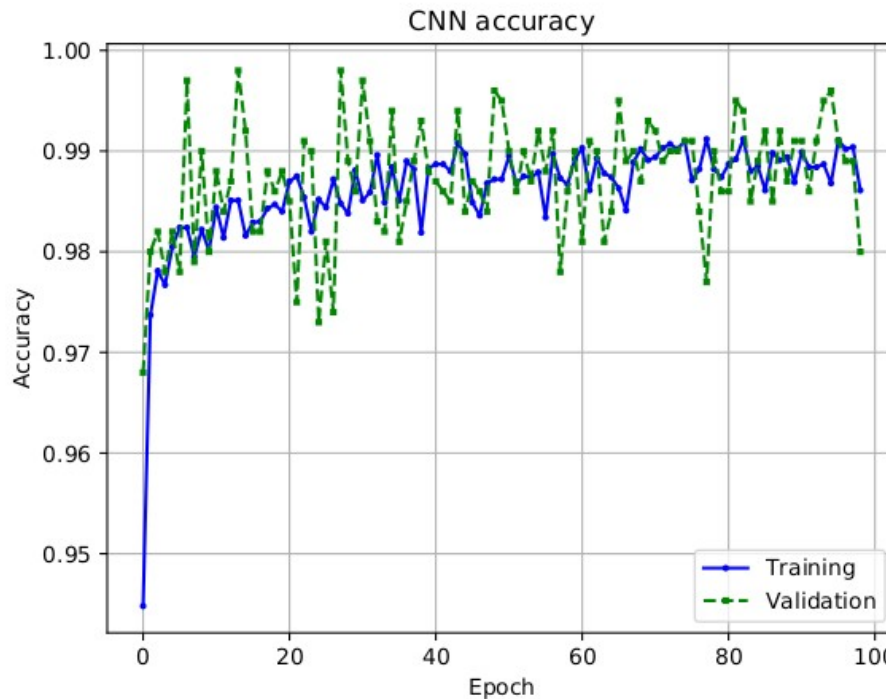
System Calls
