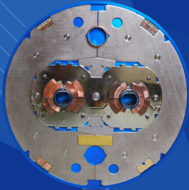
LHC dipole cross-section
