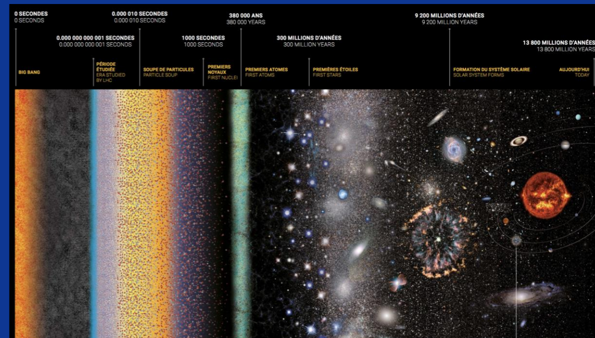
Cosmic evolution
