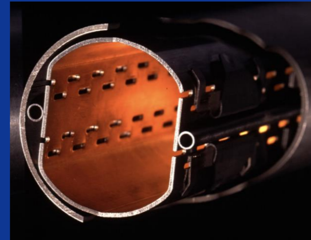
LHC beam pipe
