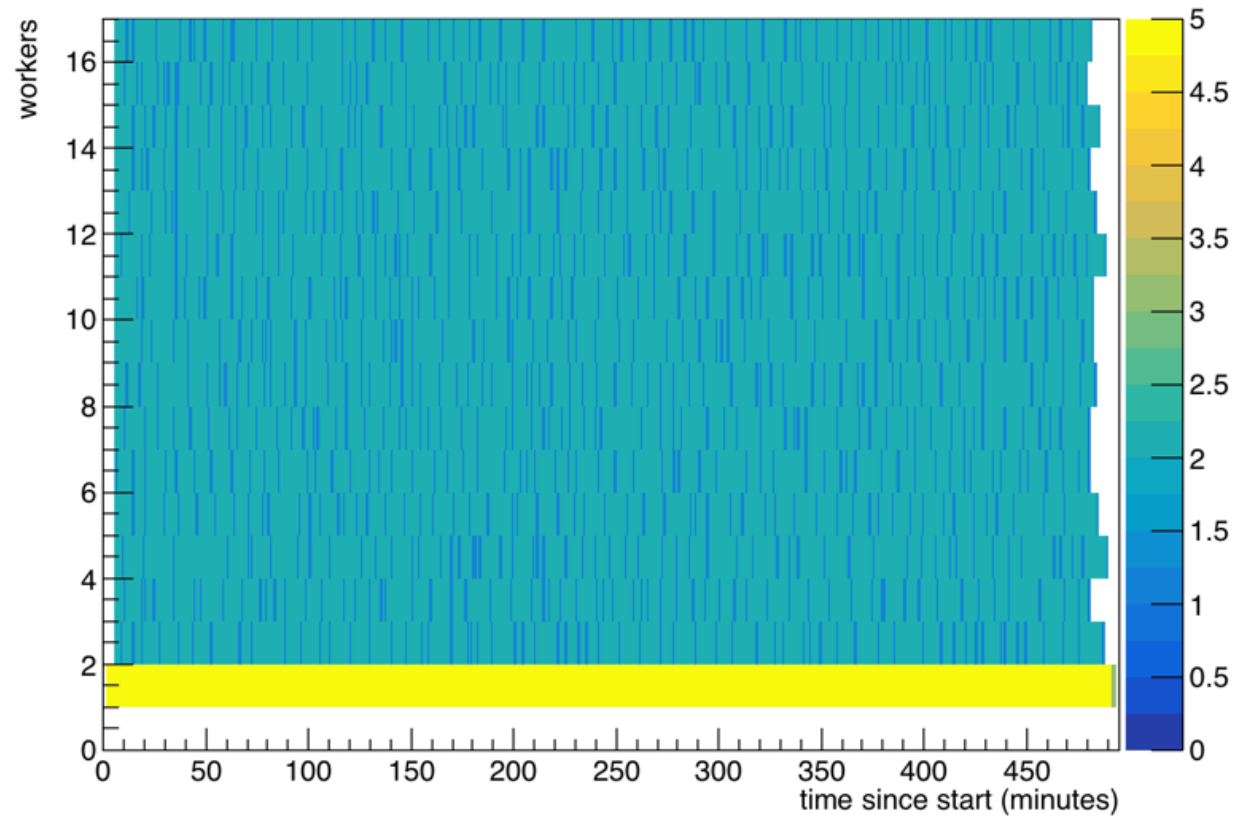
AthenaMP worker occupancy with 1k input events. Job# 3664710767
