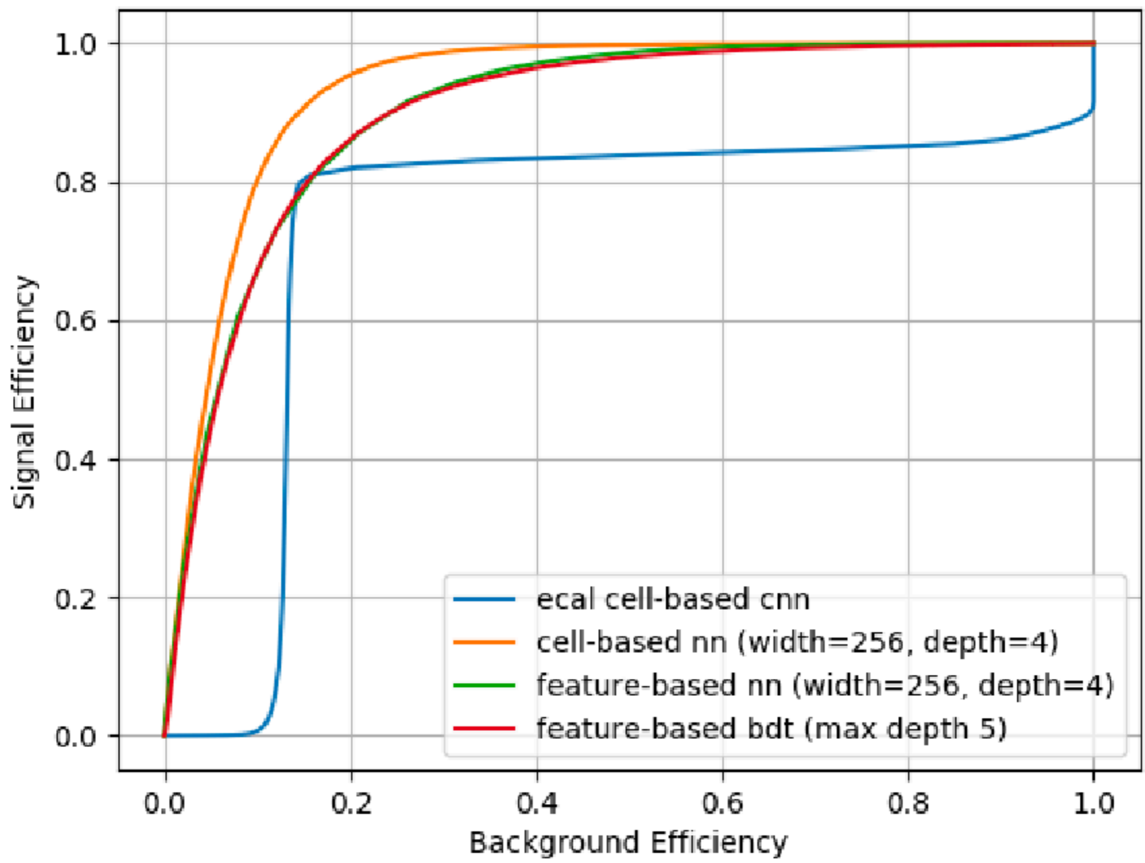
ROC for Gamma vs. Pi0 Classifier
