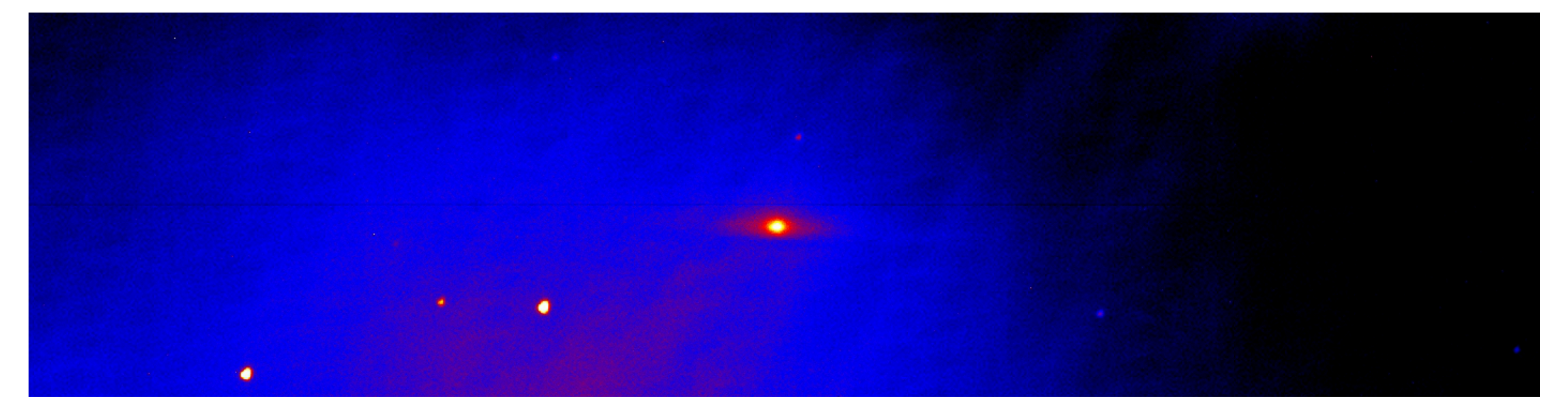
Sombrero Spiral Galaxy (M104). The red halo on the bottom left is due to a brighter object.
