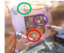
Heat load
