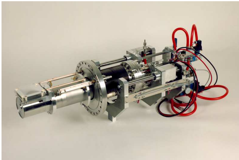
Figure 2.34: The feed-through mounted on a \text{Ø}200 mm flange containing the scintillator and IC inside the pocket at atmospheric pressure and the SEM in the vacuum.
