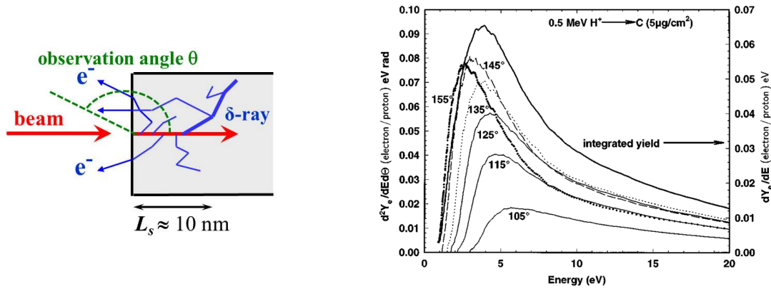
Figure 2.19: Left: Schematic drawing of the secondary electron generation from a surface by charged particle impact; L_s is the scattering length from which electrons are able to reach the surface. Right: A typical measurement of the electron energy spectrum for different emission angles and the total yield in backward direction by 0.5 MeV proton impact on a carbon foil, from [17].
