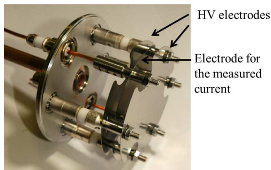
Figure 8.5: Photo of a three plate SEM beam loss monitor [147].
