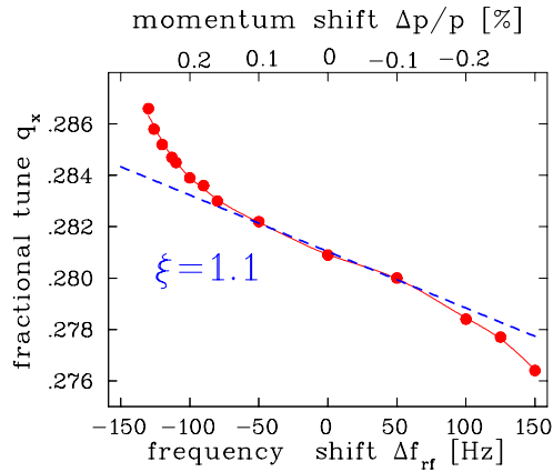
Figure 5.39: Measurement of the chromaticity at LEP. The horizontal tune is determined for different setting of the acceleration frequency and therefore of the momentum of the circulating beam. The chromaticity is fitted through the linear part of the data [121].
