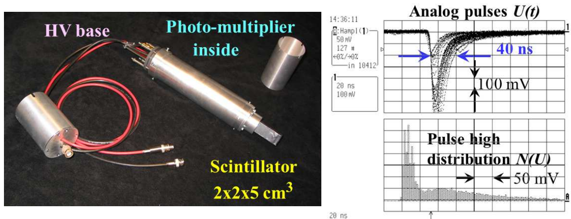
Figure 8.4: Left: Photo of a typical BLM based on a plastic scintillator connected to a photo-multiplier. Right: Typical pulses from a plastic scintillator (top, 100 mV/div and 20 ns/div) and their pulse height distribution (bottom, 50 mV/div) as measured at the GSI heavy ion synchrotron.
