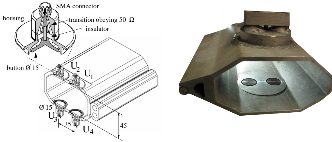
Figure 5.16: Left: Typical button BPM arrangement within a vacuum chamber at a synchrotron light source, from [93]. Right: Photo of the realization at HERA, DESY.
