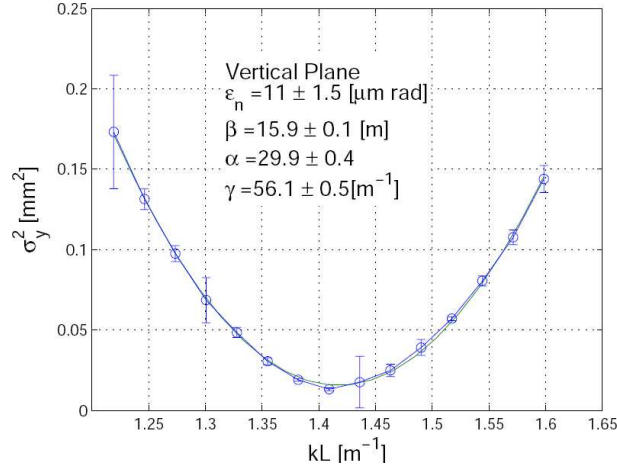
Figure 4.9: Profile width determined with a YAG:Ce screen at Elettra electron LINAC for a quadrupole variation and the parabolic fit, from [79].
