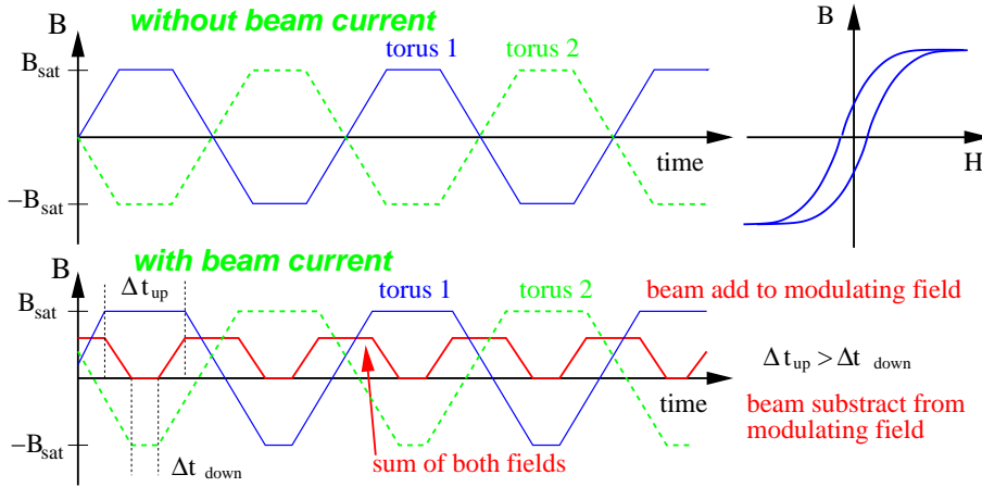
Figure 2.13: The fluxes in the two tori of a dc-transformer without and with a beam. The magnetic field of the beam adds to the modulated field for one modulation phase and 180^\circ degree later it is subtracted. The sum of the maximum magnetization gives the measured signal. The scheme is drawn for a triangular-modulation, for a realistic sine-modulation the edges are smoother.
