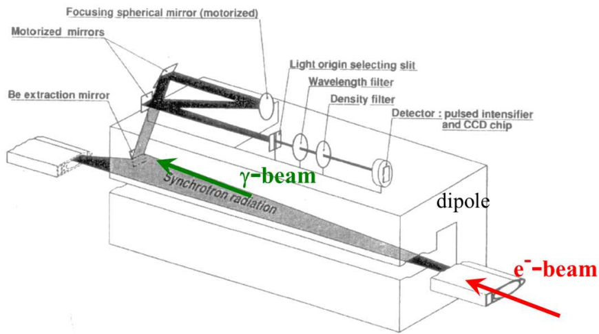
Figure 3.28: The synchrotron radiation profile monitor at LEP. The optical system is installed close to the 23 m long dipole magnet with bending radius of 3100 m, from [68].
