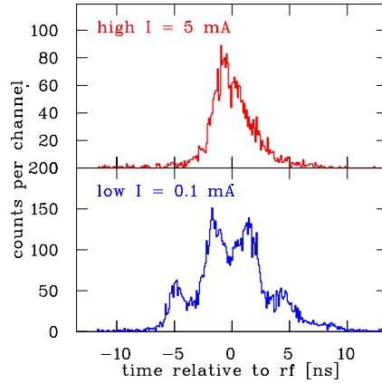
Figure 6.21: The bunch structure measured at the GSI LINAC with a 120 keV/u \text{Ar}^{1+} beam for different currents inside the RFQ [78]; one rf-period is shown.
