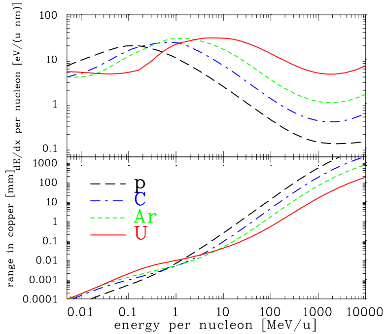
Figure 2.17: The energy loss per nucleon at the surface and the range in copper as a function of the kinetic energy for several ions. The energy range is plotted from 5 keV/u to 10 GeV/u and the range from 100 nm to 1 m. The calculation of the electronic and nuclear stopping uses the semi-empirical code SRIM [13].
