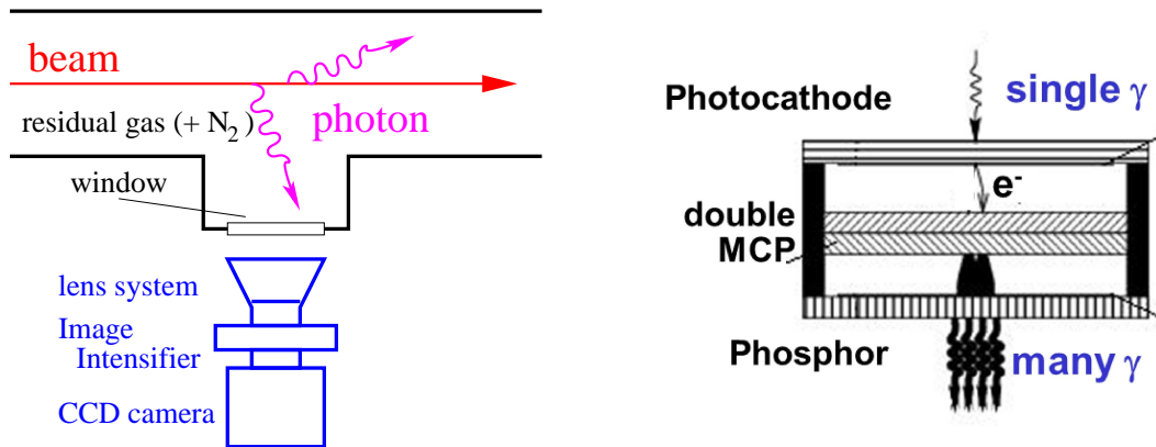
Figure 3.20: Left: General scheme of the profile determination via detection of the residual gas fluorescence. Right: Scheme of an image intensifier consisting a photo-cathode, a MCP and a phosphor screen.
