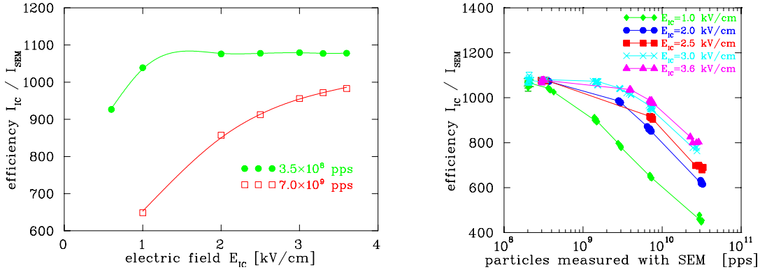
Figure 2.37: Left: The characteristic line for the IC as determined of the 300 MeV/u Ne 10+ beam. The efficiency, as measured by the ratio of the secondary current of the IC and the SEM as a function of the applied electric field [20]. For a low primary current a plateau is reached, while for a high current the recombination leads to a decrease of the secondary charges. Right: Comparable data shown as a function of transmitted ions per second for different applied electric field.
