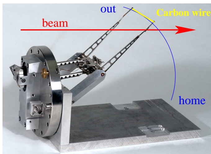
Figure 3.8: Pendulum scanner or 'flying wire' used at CERN synchrotron [38].
