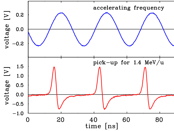
Figure 6.3: The LINAC module accelerating frequency (top) and the corresponding pick-up signal recorded by a capacitive pick-up (bottom) for the determination of the bunch zero crossing from a 1.4 MeV/u ion beam.
