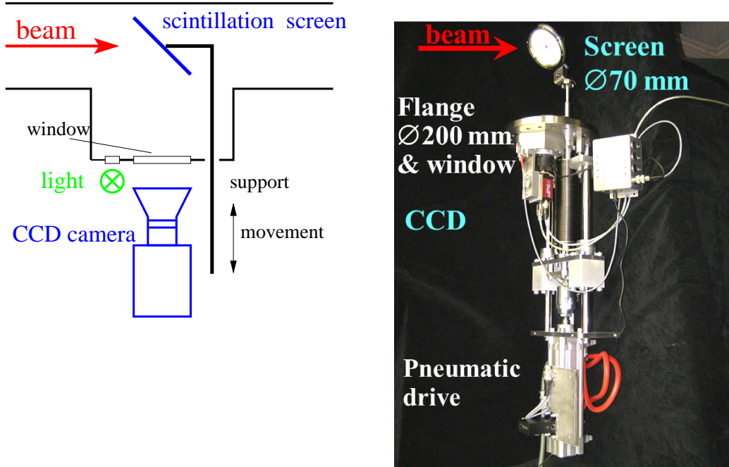
Figure 3.1: Left: The scheme of an intercepting scintillation screen is shown. Right: A photo from a P43 phosphor scintillation screen of \text{Ø}70 mm and the CCD camera are mounted on a \text{Ø}200 mm flange with pneumatic drive is depicted.
