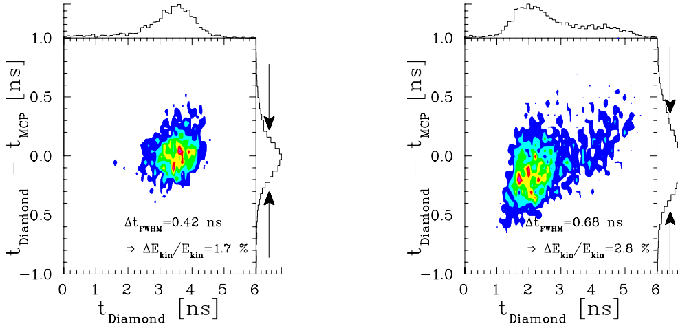
Figure 6.22: Phase space plot for a 1.4 MeV/u ion beam recorded with two detectors in coincidence at the GSI LINAC [78]. The time relative to the rf is plotted along the horizontal axis, the time difference of the individual particles on the vertical axis corresponding to the energy distribution. Left: The low current ( I_{beam} = 0.1 mA) results are plotted. Right: The high current beam ( I_{beam} = 5 mA) results is depicted.
