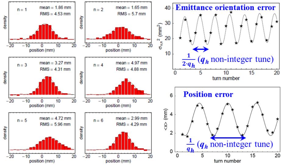
Figure 3.7: Left: Profile measurement for a mismatched injection into the CERN PS synchrotron for the first n = 1 \dots 6 turns Right: Fitted square of the beam width and centre as a function of time, from [44].
