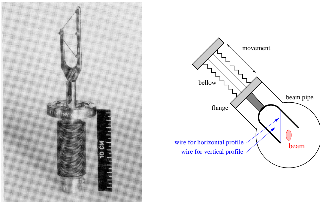
Figure 3.10: Linear scanner used at CERN [41].
