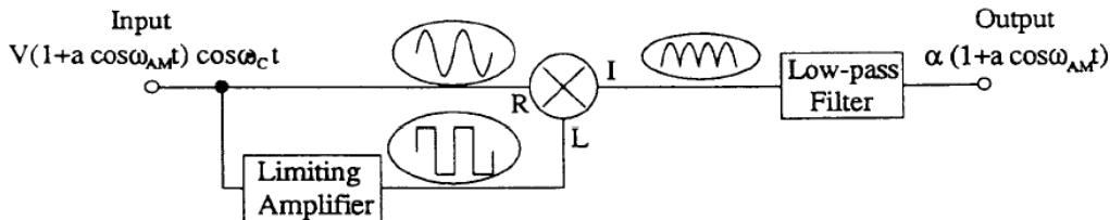
Figure 5.28: Scheme of a synchronous detector to rectify an rf signal.
