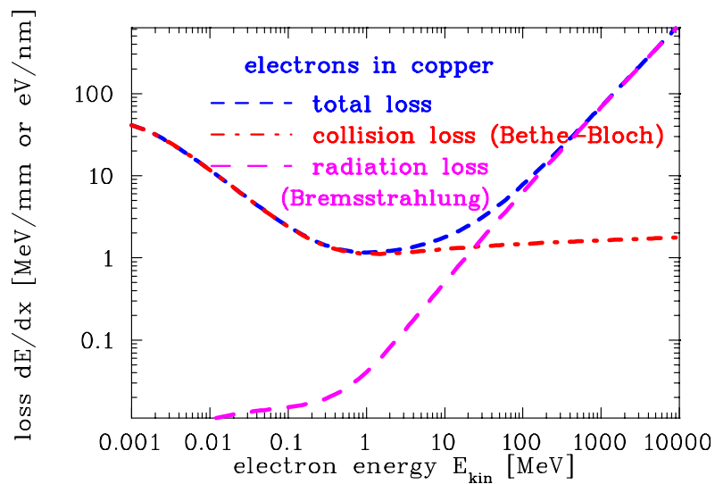
Figure 2.18: The energy loss of electrons in copper for collision loss as given by the Bethe-Bloch equation and radiation losses as dominated by the emission of Bremsstrahlungs-photons, data from [15].
