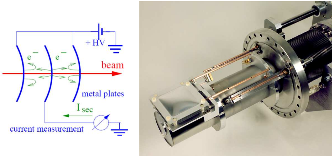
Figure 2.38: Left: Scheme of a SEM made of three metal foils. Right: Photo of the SEM part made of 3 Al foils with thickness of 100 \mu\text{m} of the feed-through used for slow extraction at GSI.
