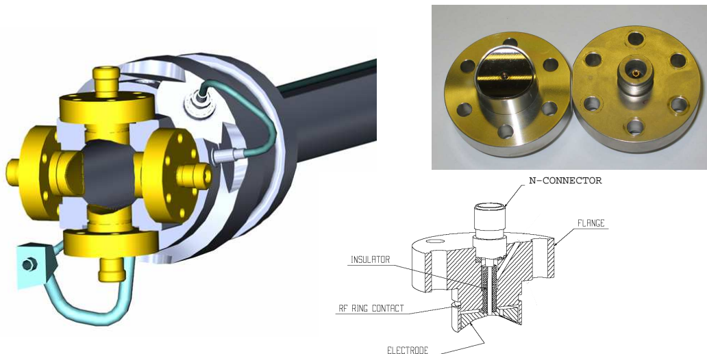
Figure 5.15: Left: The installation of the curved \text{\O} 24 mm button BPMs at the LHC beam pipe of \text{\O} 50 mm, from [92]. Right: Photo of a BPM used at LHC, the air side is equipped with a N-connector as well as a technical drawing for this type.
