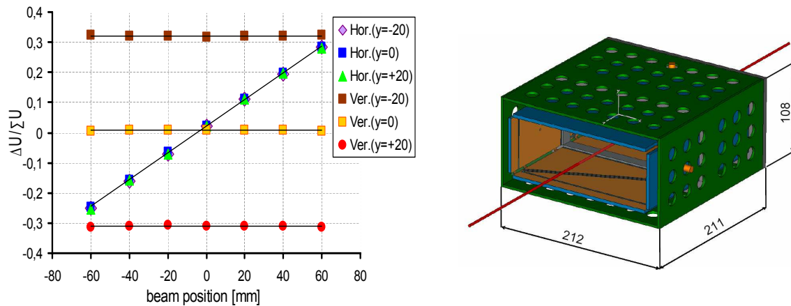
Figure 5.20: Left: Numerical calculation of the position reading \Delta U/\Sigma U as a function of beam displacement for the horizontal plane. The the simulated beam is swept in horizontal direction (curves with constant slope) and vertical direction (constant functions) and proves the decoupling of both planes [97]. Right The BPM geometry for these calculations is depicted right having a horizontal half-aperture of a = 100 \text{ mm} and vertical half-aperture of b = 35 \text{ mm} and a length of 211 \text{ mm} comparable, to the one shown in Fig 5.19.
