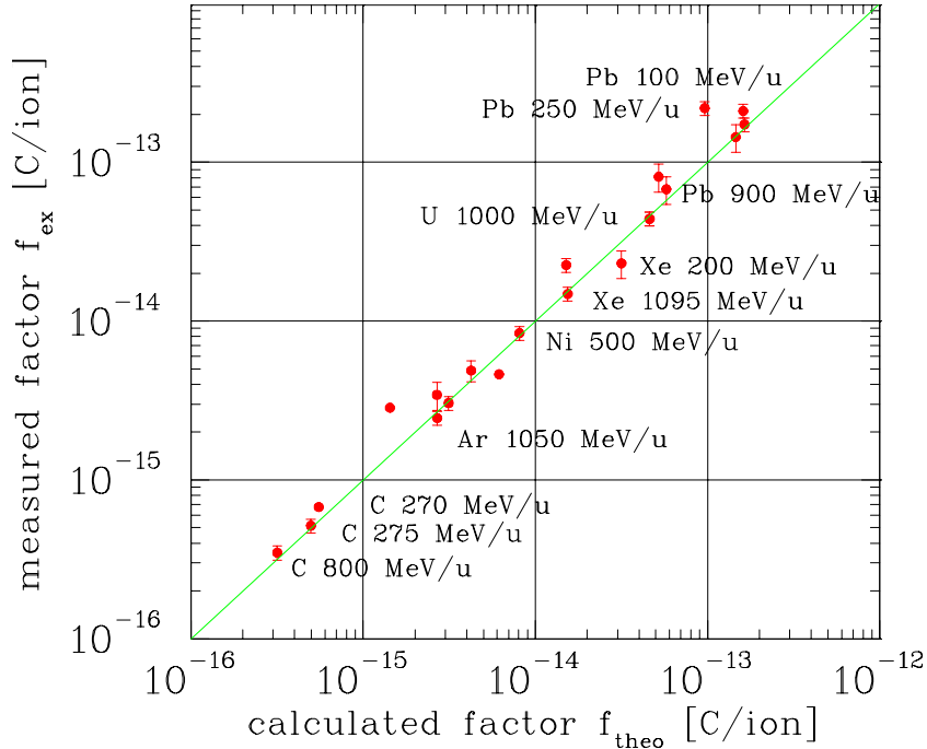
Figure 2.36: The measured calibration factor of an IC and calculated value using energy loss for various slowly extracted ions from the GSI synchrotron [21].
