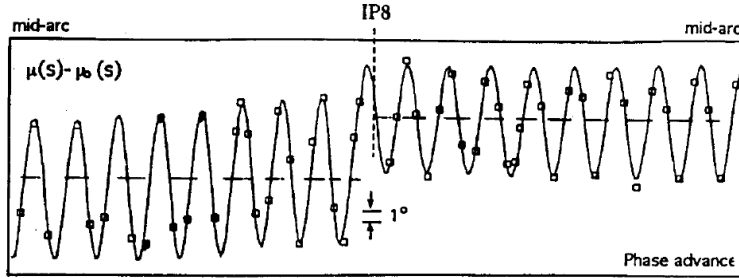
Figure 5.37: Scheme of the individual measurements at two pick-ups for a phase advance \Delta\mu determination. A sine function can be fitted through the data points.
