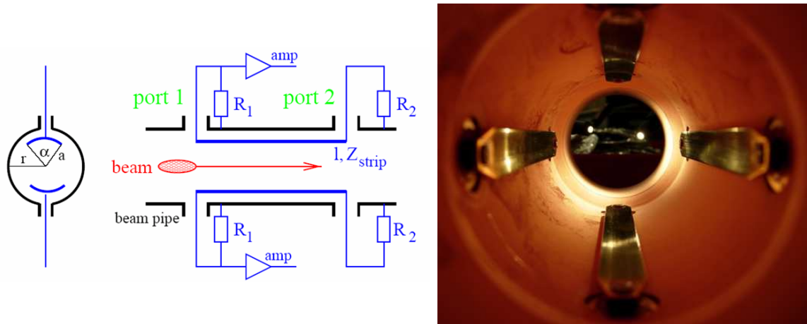
Figure 5.21: Left: Scheme of a stripline pick-up. Right: Photo of the LHC stripline BPM of 12 cm length, from [92].
