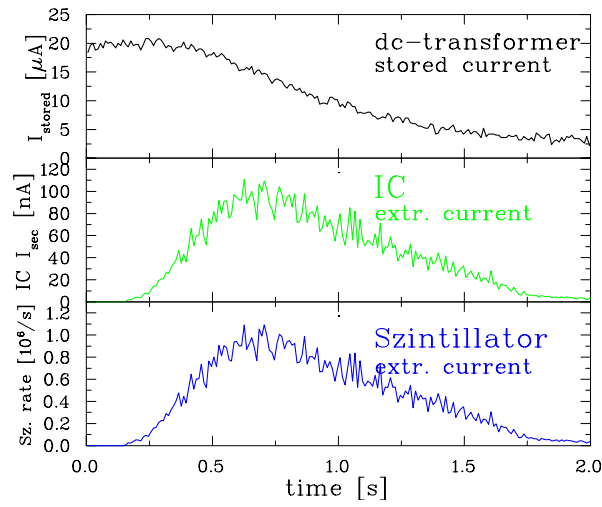
Figure 2.33: The extracted current measured by an IC (middle, given in nA for the secondary current) and a scintillator (bottom, given in particles per second) as compared to the current inside the GSI synchrotron determined by a dc-transformer (top, given in \mu\text{A} ) for one extraction of a 250 MeV/u ^{208}\text{Pb}^{67+} beam with a total amount of 10^6 particles.
