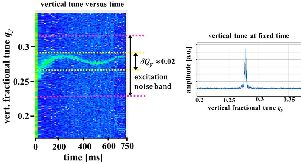
Figure 5.36: Left: Measurement of the tune at the GSI synchrotron for an \text{Ar}^{10+} beam accelerated from 11 to 300 MeV/u within 0.75 s [117]. Displayed is the Fourier transformation of displacements of successive individual bunches over 4096 turns excited by the depicted noise band during acceleration as a function of time. The maximum of the Fourier transformation is color-coded in a linear manner; \delta Q_y is the variation of the tune value. Right: Single tune spectrum 110 ms after the ramp start averaged over 4096 turns corresponding to \sim 15 ms.
