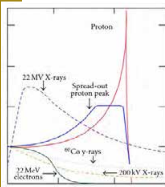
Fig. 3.5: The relative dose as a function of depth for X-rays (photons), electrons and protons in water. A proton beam at a fixed energy produces the red curve, ending in the so-called Bragg peak. This can be spread out over the tumour volume by overlapping the dose created from multiple beams with different proton energies and fluence, the sum of which is called the spread-out Bragg peak (SOBP) (credit: M. Cianchetti, Int. J. Otolaryngology, 2012, 3, 325891, CC BY 3.0.)
