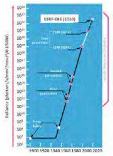
Fig. 7.2: The evolution of the peak brilliance of electron storage rings (credit: ESRF).
