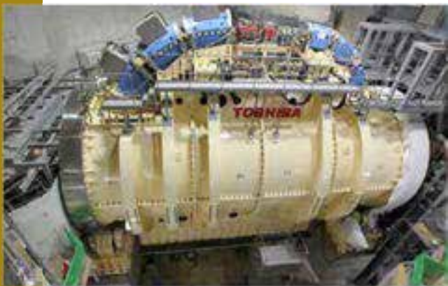
Fig. 3.11: The first superconducting gantry for carbon-ion therapy, installed at NIRS (Japan), which utilises superconducting, combined-function magnets with fields up to 2.9 T (credit: Y. Iwata/NIRS).
