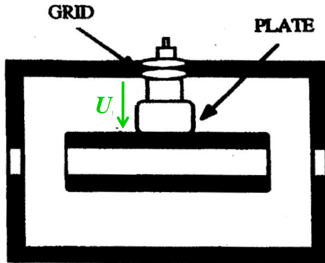
"Wideroe" or \lambda/2 structure
