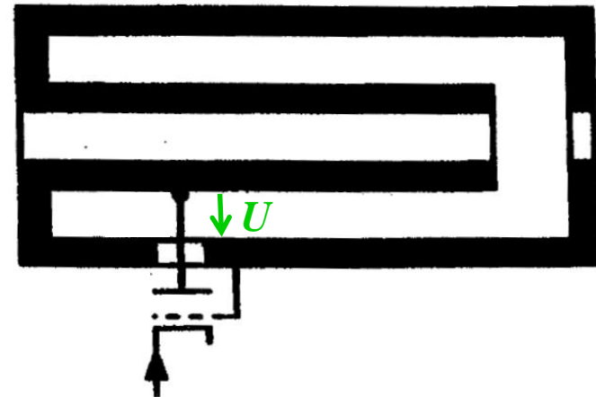
basic \lambda/4 - resonator
