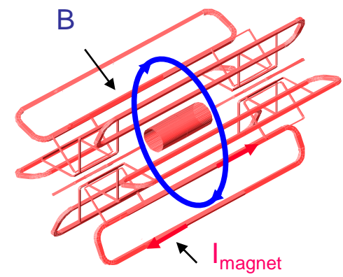
(air-core) Toroide
