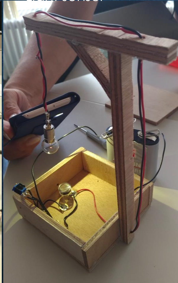
Light sensor
