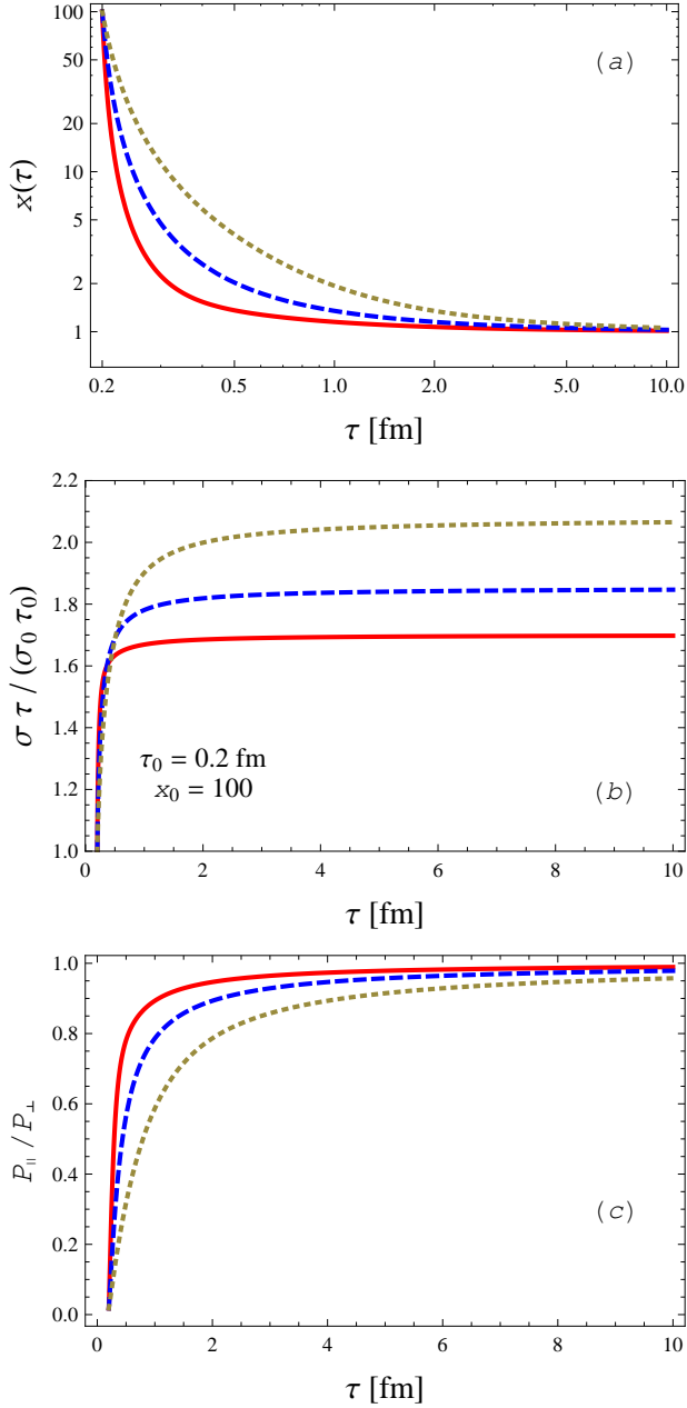
Figure 1: (a) Time dependence of the asymmetry parameter x for three different choices of the relaxation time: \tau_{\text{eq}} = 0.25 fm (solid line), \tau_{\text{eq}} = 0.5 fm (dashed line), and \tau_{\text{eq}} = 1.0 fm (dotted line). (b) Entropy density divided by the corresponding values obtained in the Bjorken model. (c) Ratio of the longitudinal and transverse pressures shown as a function of the proper time. All results are obtained with the initial asymmetry x_0 = 100 .
