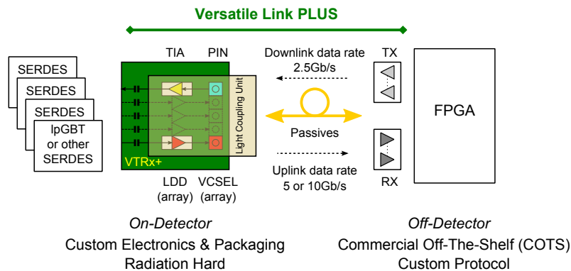
Figure 1: The Versatile Link + architecture.
