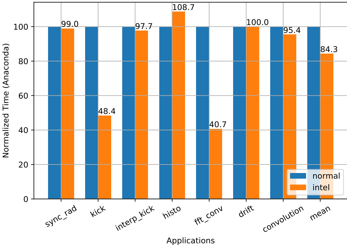
Runtime comparison of the Intel and Anaconda distribution
