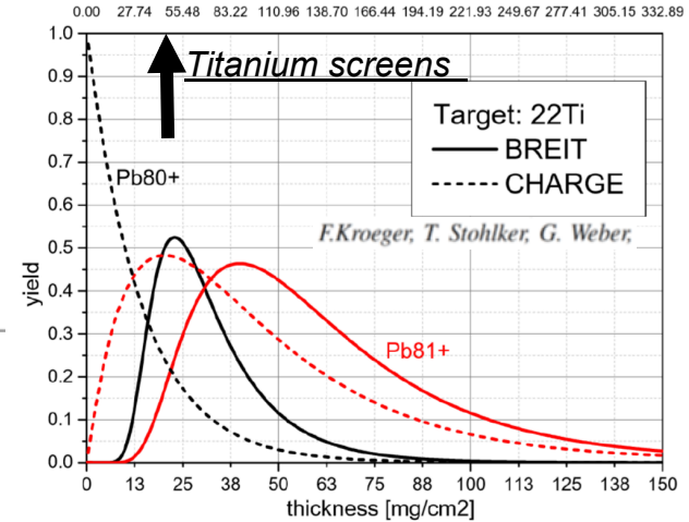
Pb54+ on 22Ti with 5900MeV/u thickness [ \mu\text{m} ]
