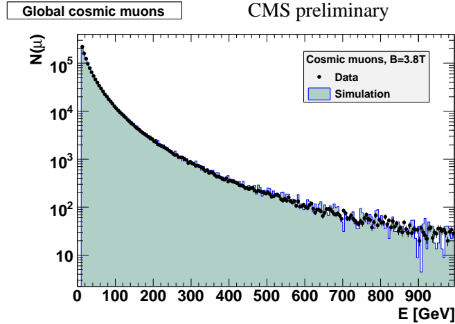
Fig. 2: Energy spectrum of muons in data (black points) measured with the CMS detector. In comparison the GEANT simulation (green/blue histogram) is shown. The simulation has been normalised to the number of events of the data.
