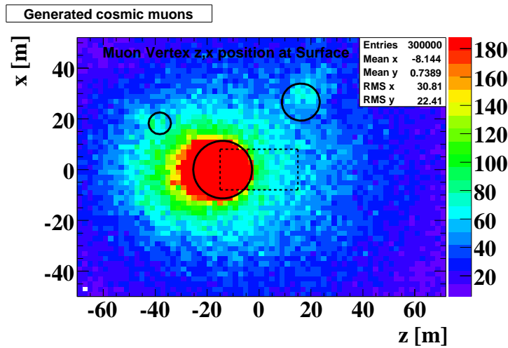
Fig. 1: Entrance vertex at the surface of the generated muons which arrive at the CMS detector (indicated by the dashed rectangle) 90 m underground. The three vertical shafts are indicated by black circles. There is clearly a correlation between muon intensity and shafts visible.
