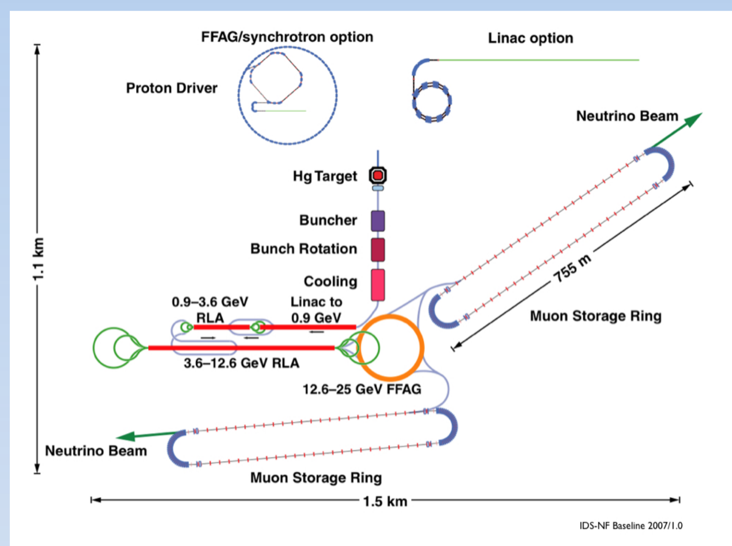
Fig. 1: The Neutrino Factory layout
