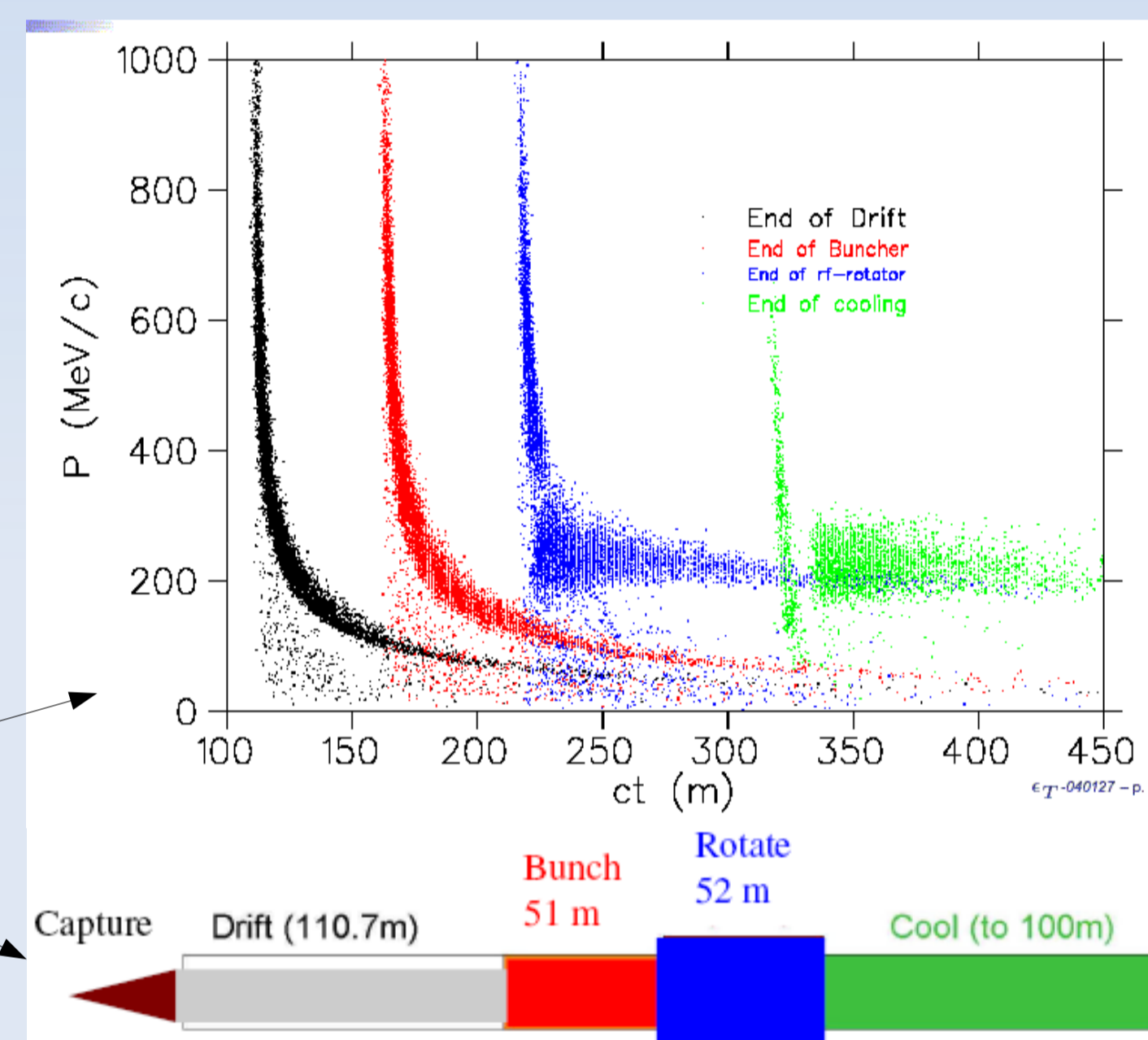
Fig. 1: The Neutrino Factory layout
