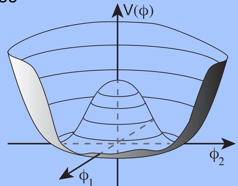
Higgs - Potential
