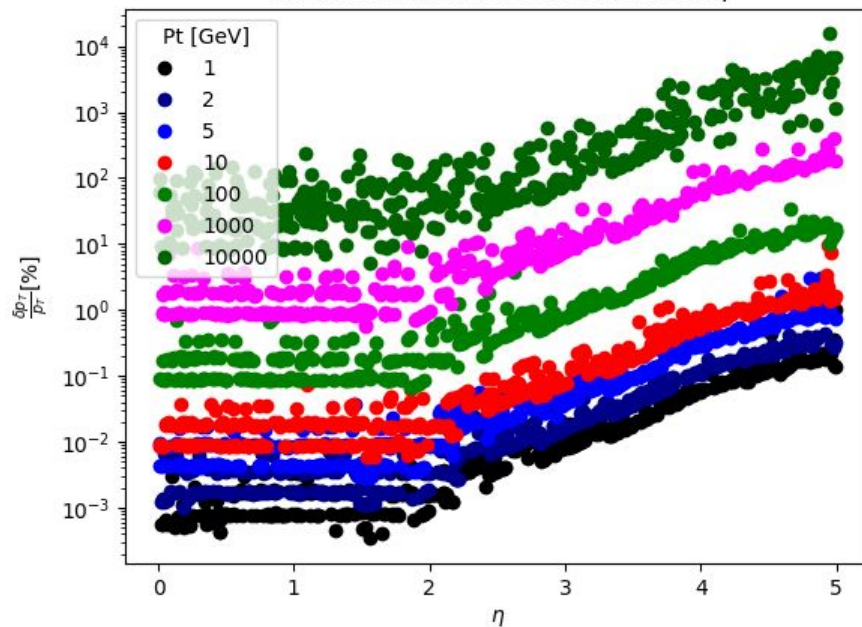
Track resolution for const Pt across \eta
