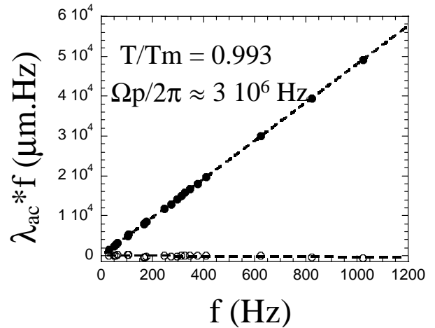
Fig. 5. The low frequency response of the vortex lattice \lambda_{ac} \times f as function of the frequency f , so as to emphasize the low frequency linearity which implies \lambda' \simeq 48.5 \mu\text{m} < \ell_a/2 .
