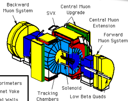
CDF Detector
