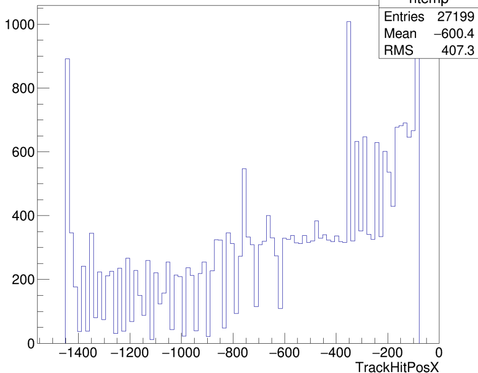
TrackHitPosX {MCTrkID==0}
