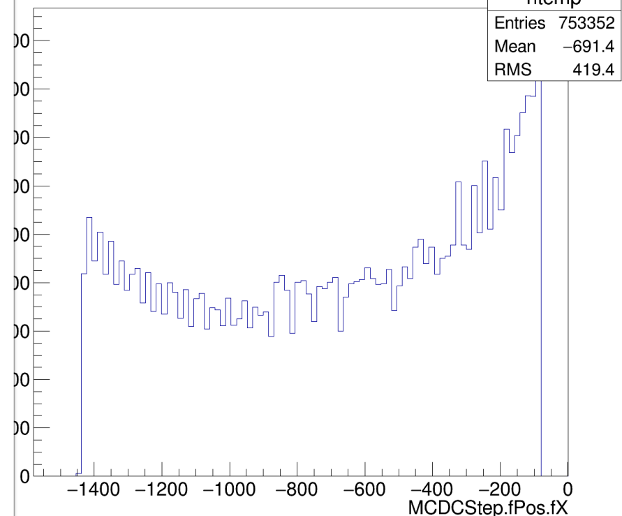
MCDCStep.fPos.fX {MCDCStep.fTrackID==1}
