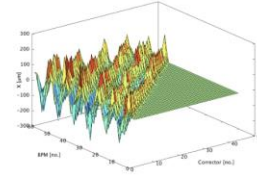
Fig. 6: The orbit response matrix, R, as measured by estimating the orbit difference from systematic alternating-sign correctors kicks and applying the system identification algorithm.
