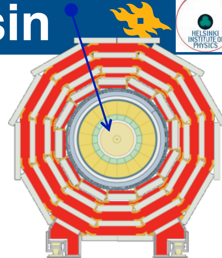
Run 50905 Event 1576, y vs x
