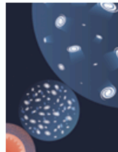
Cosmic acceleration
