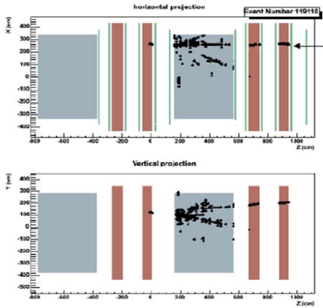
CC event in the first magnet
