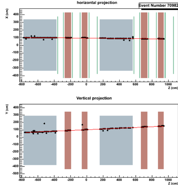
Muon from CC interaction in the material in front of the detector (BOREXINO, rocks)
