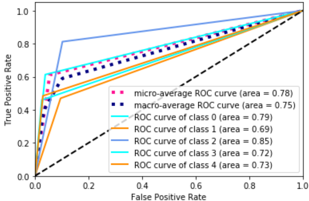
(a) Receiver Operator Characteristic (ROC) curve
