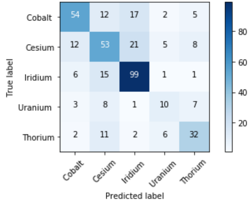
(b) Confusion matrix
