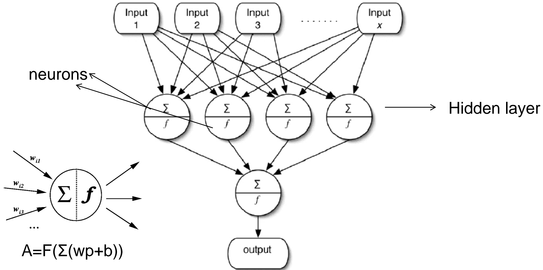
Fig. Structure of a 2 layer neural network
