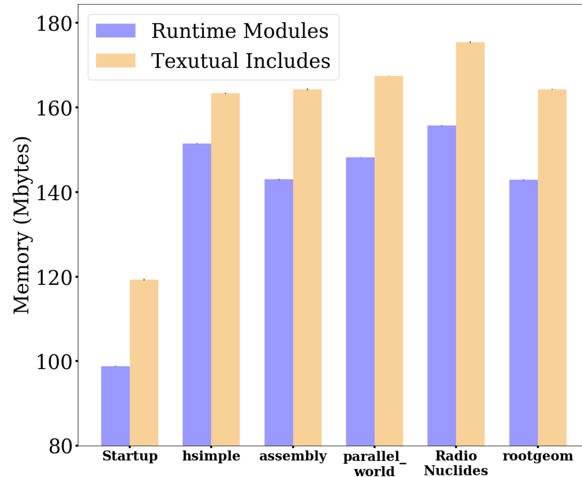
Figure 4: Residential memory used to run tutorials.
