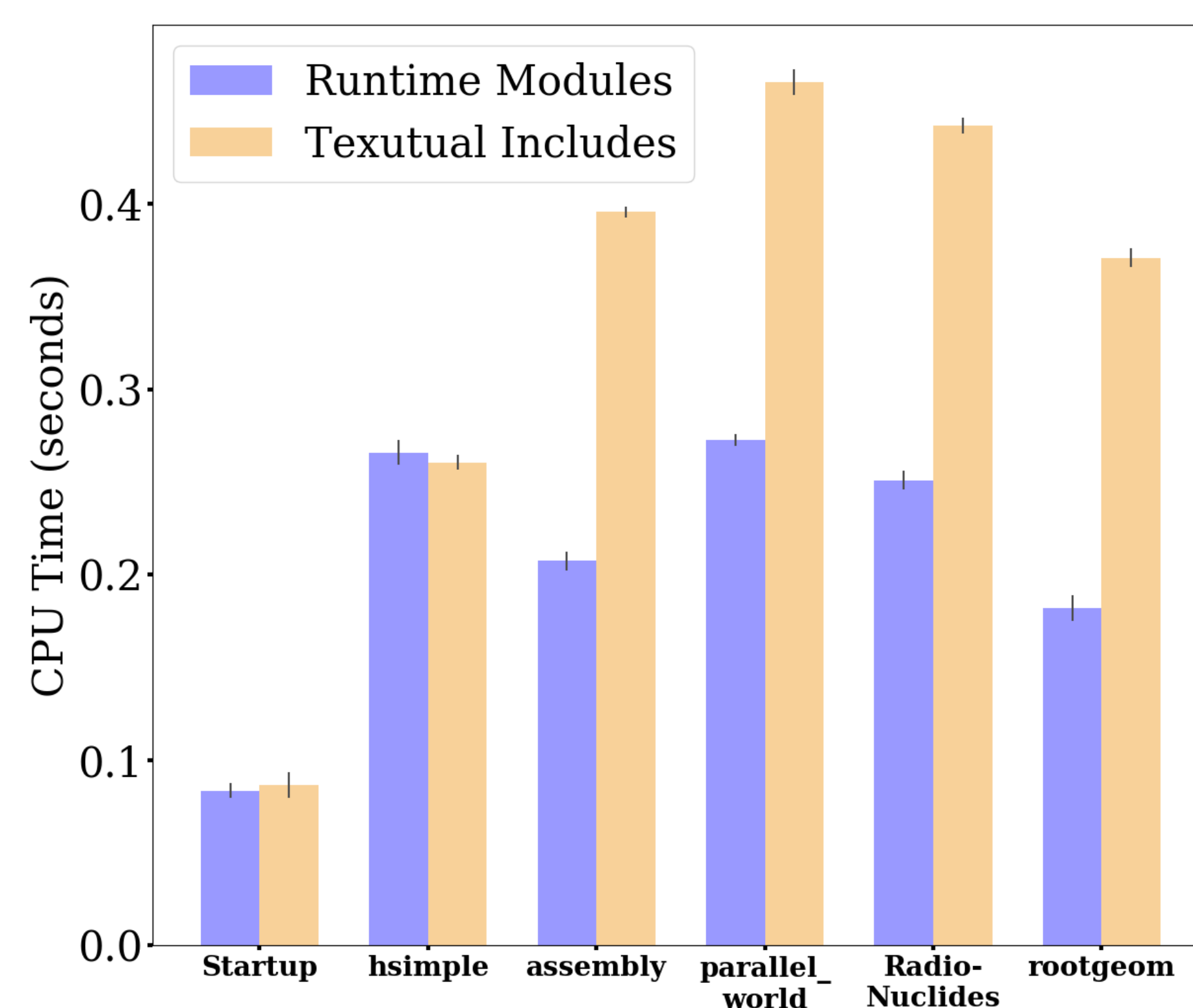
Figure 3: CPU Time required to run selected tutorials. The first column is displaying ROOT's time to start into an empty shell.
