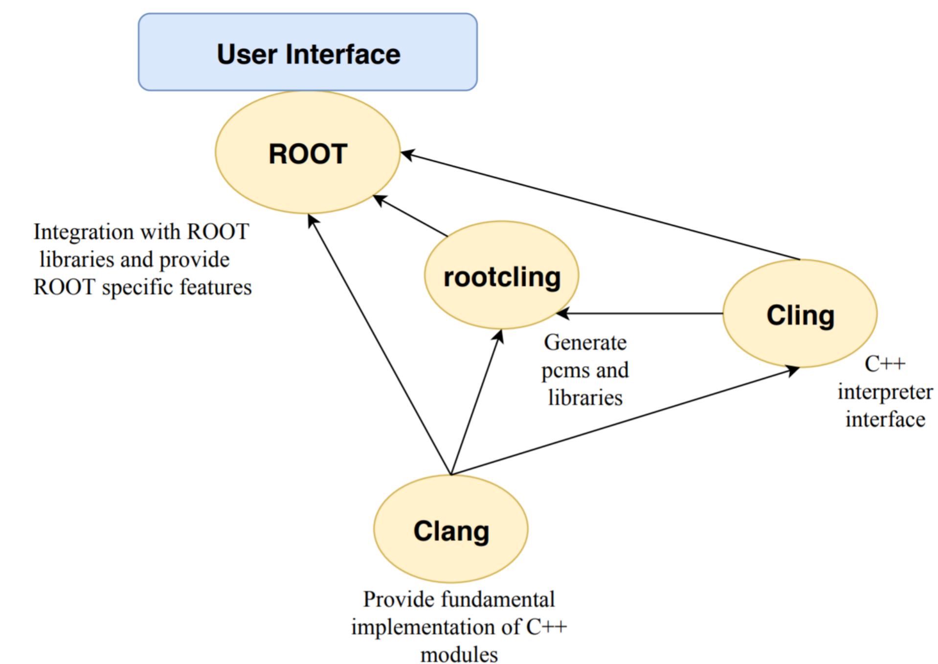
Figure 5: Visualization of ROOT interpreter core.
