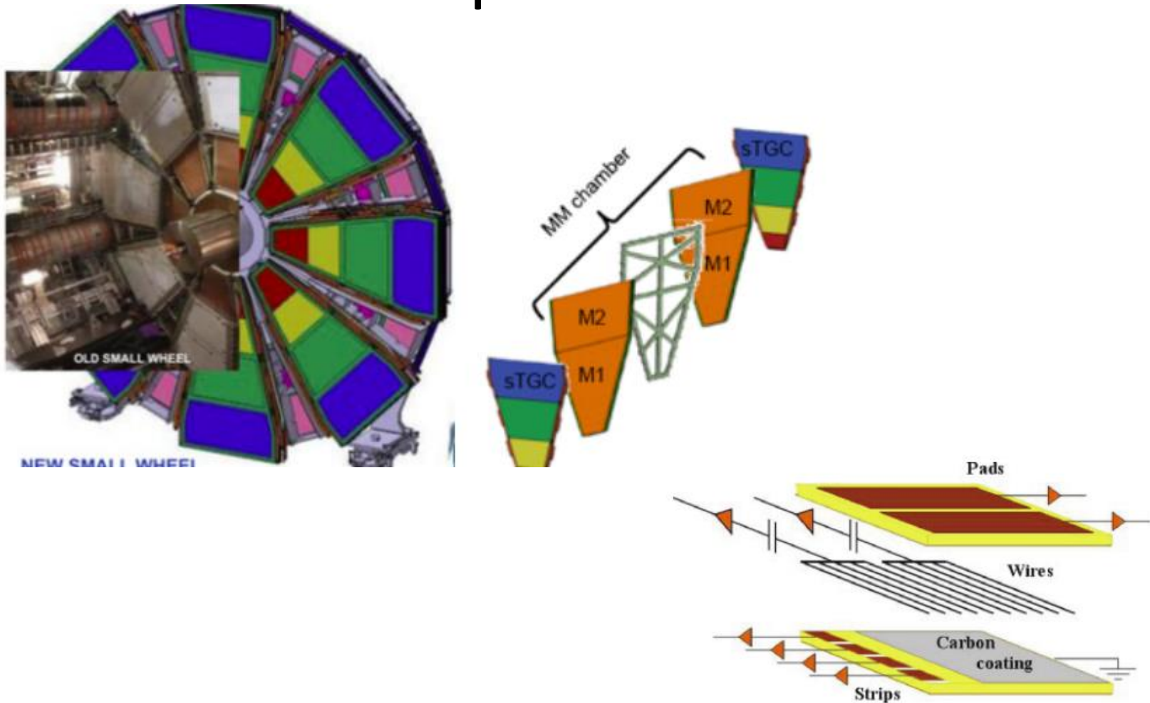
Figure 5: Schematics of the basic sTGC structure.
