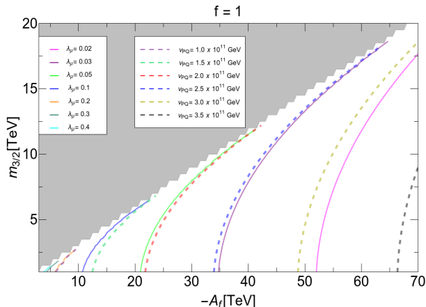
Figure 5: Representative values of \lambda_\mu required for \mu = 200 GeV in the m_{3/2} vs. -A_f plane of the hyCCK model for f = 1 . We also show several contours of v_{PQ} .
