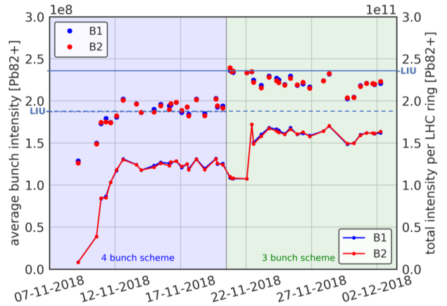
Figure 3: Average bunch intensity (points and left vertical axis) and total beam intensity (solid lines and right vertical axis) per LHC fill as a function of time during the 2018 Pb-Pb run. The LIU goals for both are also shown as horizontal lines (dashed for bunch intensity and solid for total beam intensity).
