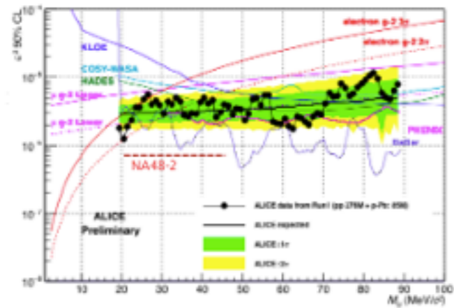
Fig. 11: 90% of CL constrained by ALICE
