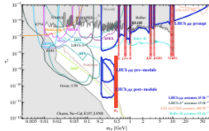
Fig. 14: 90% of CL constrained by LHCb in HL-LHC era
