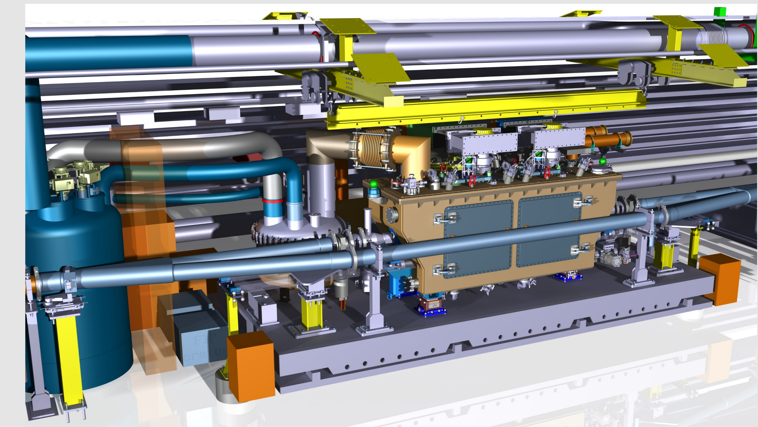
Information about DQW cryomodule
