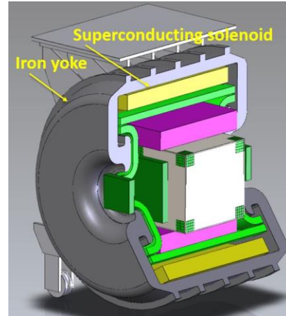
Fig. 6 KLOE superconducting magnet system.
