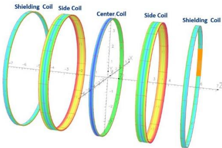
Fig. 2 The HPgTPC detector superconducting coils configuration.
