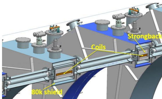
Fig. 8. Cross sectional view of coils assembly.
