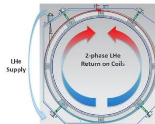
Fig. 10 Thermosyphon coil cooling.
