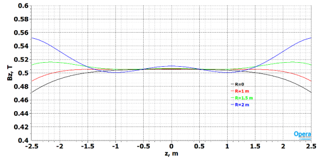
Fig. 3 Magnetic field in the magnet bore.
