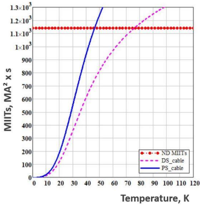
Fig. 5 Superconducting cables adiabatic heating during quench.
