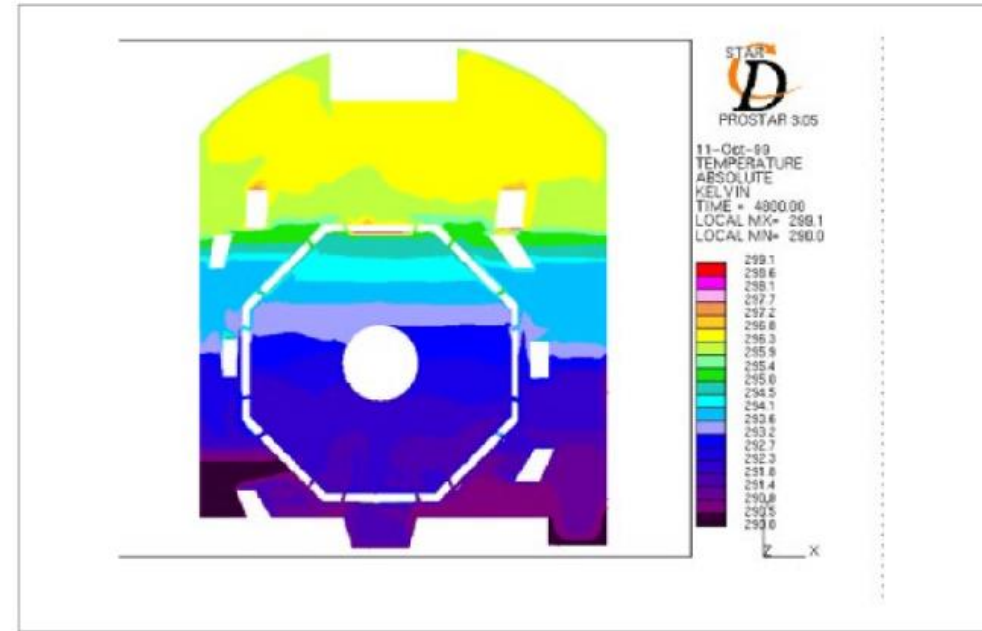
Temperature distribution
