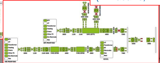
GUI of the Fast Beam Investigation (FBI) software (E. Fadakis, E. Matli, BE-OP-ISO)
