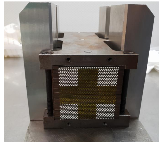
Prototype module containing cells made with variety of fibre materials, incld. GAGG.
