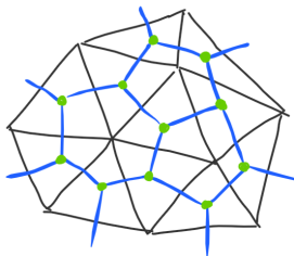
2D slice and its dual graph
