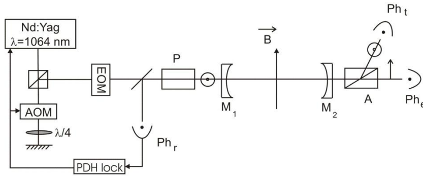
Fig. 1. Experimental setup of the BMV project.
