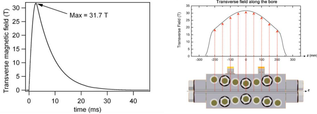
Fig. 2. XXL-Coil Left: magnetic field pulse of the XXL-Coil as a function of time. Right: measured magnetic field profile along the longitudinal axis.
