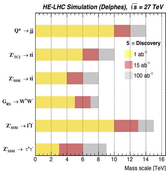
Figure 1: Discovery reach for heavy resonances.
