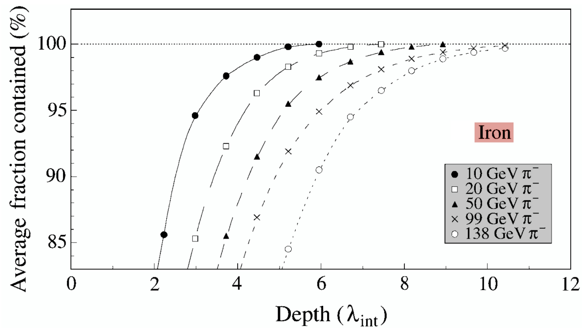
FIG. 2.43. Average energy fraction contained in a block of matter with infinite transverse dimensions, as a function of the thickness of this absorber, expressed in nuclear interaction lengths. Shown are results for showers induced by pions of various energies in iron absorber. Experimental data from [Abr 81].
