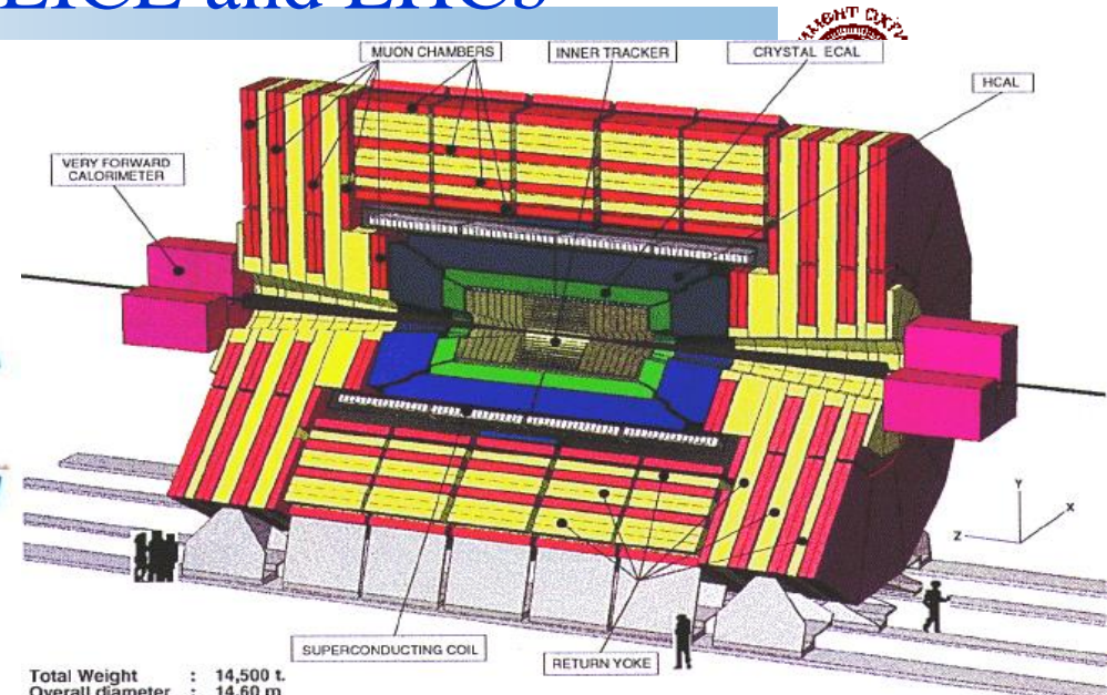
CMS – Compact Muon Solenoid
