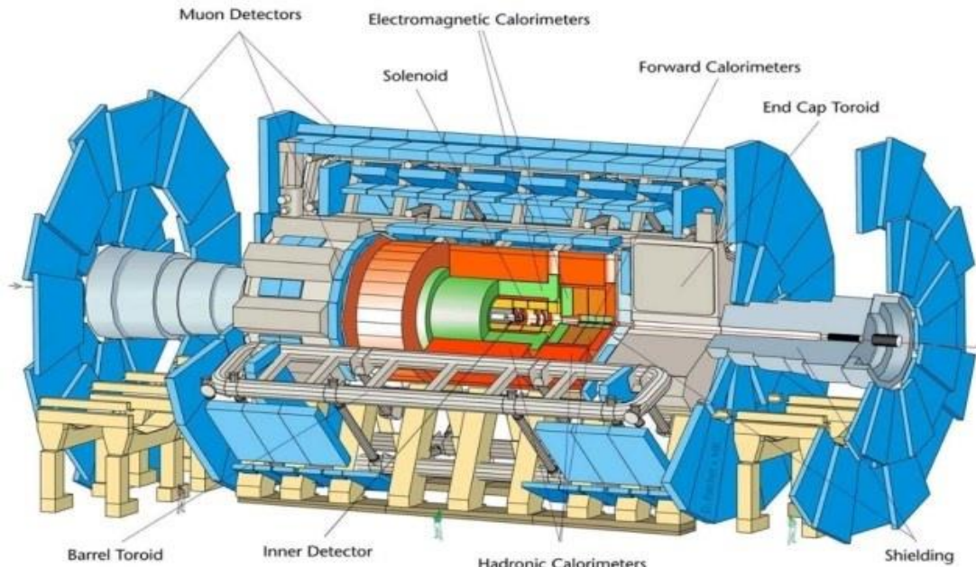
ATLAS – A Toroidal LHC Apparatus
