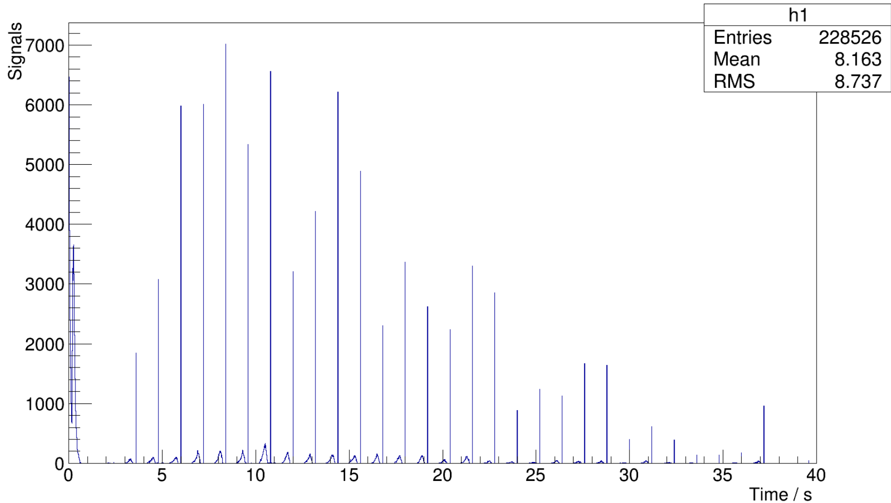
Time separation between successive beam signals in S1-3
