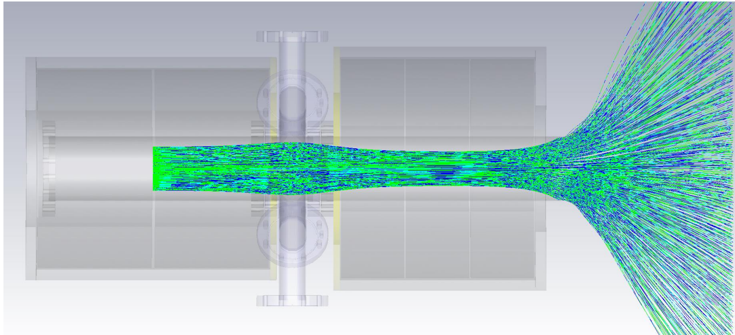
E_Path_B-Field (Ms)
