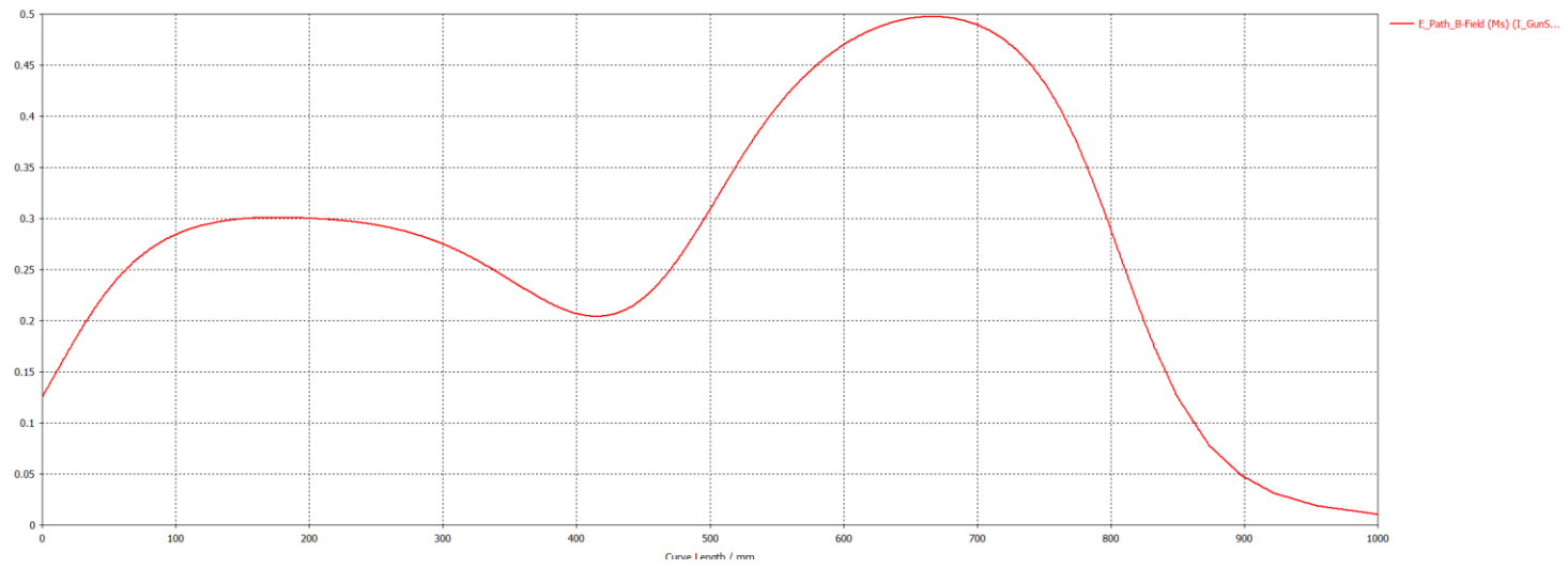
E_Path_B-Field (Ms)
